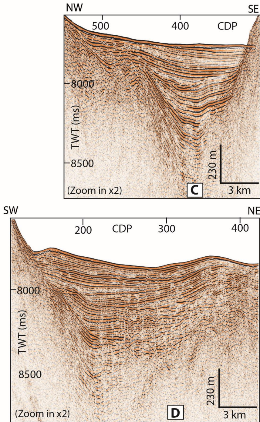
Figure 2S: Uninterpreted seismic profiles: C) Enlargement of the seismic line CAS108 (Fig. 7A). D) Enlargement of the seismic line CAS100. The vertical exaggeration is x5 for the seismic profile.
