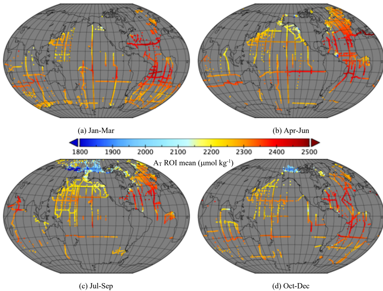
820 Figure 8. Mean A_T ( \mu\text{mol kg}^{-1} ) divided into seasons. (a) January – March (3602 ROIs); (b) April – June (3682 ROIs); (c) July – September (3960 ROIs); (d) October – December (2351 ROIs).
