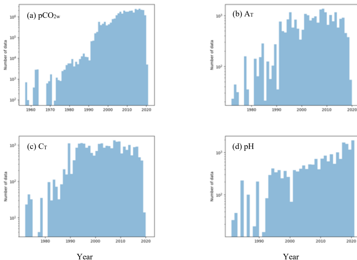
Figure 1. Numbers of carbonate system measurements included in the database per year. (a) seawater pCO_2 , (b) total alkalinity ( A_T ), (c) dissolved inorganic carbon ( C_T ), and (d) pH.
