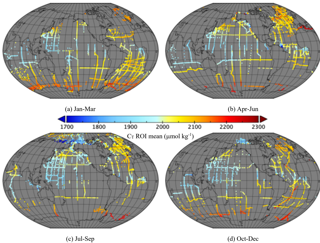
Figure 9. Mean C_T ( \mu\text{mol kg}^{-1} ) divided into seasons. (a) January – March (4029 ROIs); (b) April – June (4256 ROIs); (c) July – September (4197 ROIs); (d) October – December (2559 ROIs).
