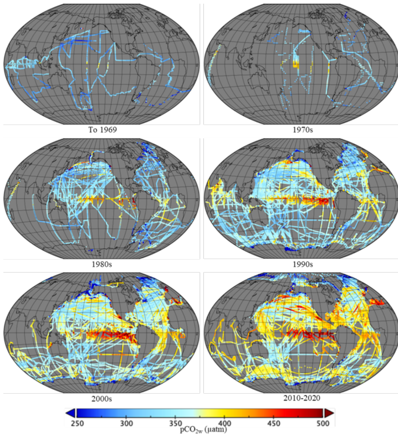
Figure 11. Mean pCO 2w (µatm) divided into decades: 1751 ROIs to 1969; 1636 in the 1970s; 9090 in the 1980s; 42,548 in the 1990s; 97,313 in the 2000s; 120,415 from 2010 to 2020.
