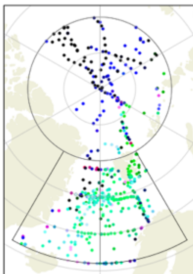
860 Figure 17. T14 regions 1 (West GIN Sea, bottom left), 2 (East GIN Sea, bottom right) and 3 (High Arctic, top) with corresponding MDB data. Each point is coloured according to the probability density of a Gaussian with mean equal to the T14 regression and standard deviation equal to its quoted RMSE, which is a measure of how consistent the data are with the T14 fit. The red component is the consistency with the region 1 fit, green with the region 2 fit and blue with the region 3 fit.
