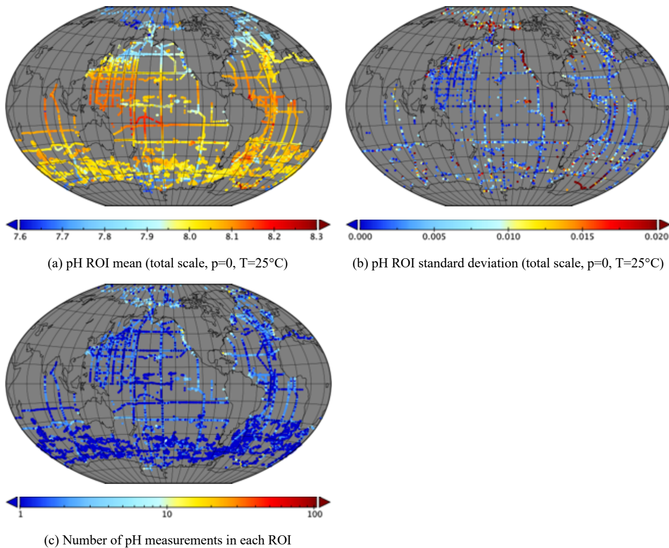
815 Figure 6. Statistics of pH in each ROI over the whole database (19,613 ROIs). (a) ROI mean, (b) ROI Standard deviation, and (c) number of measurements in each ROI.
