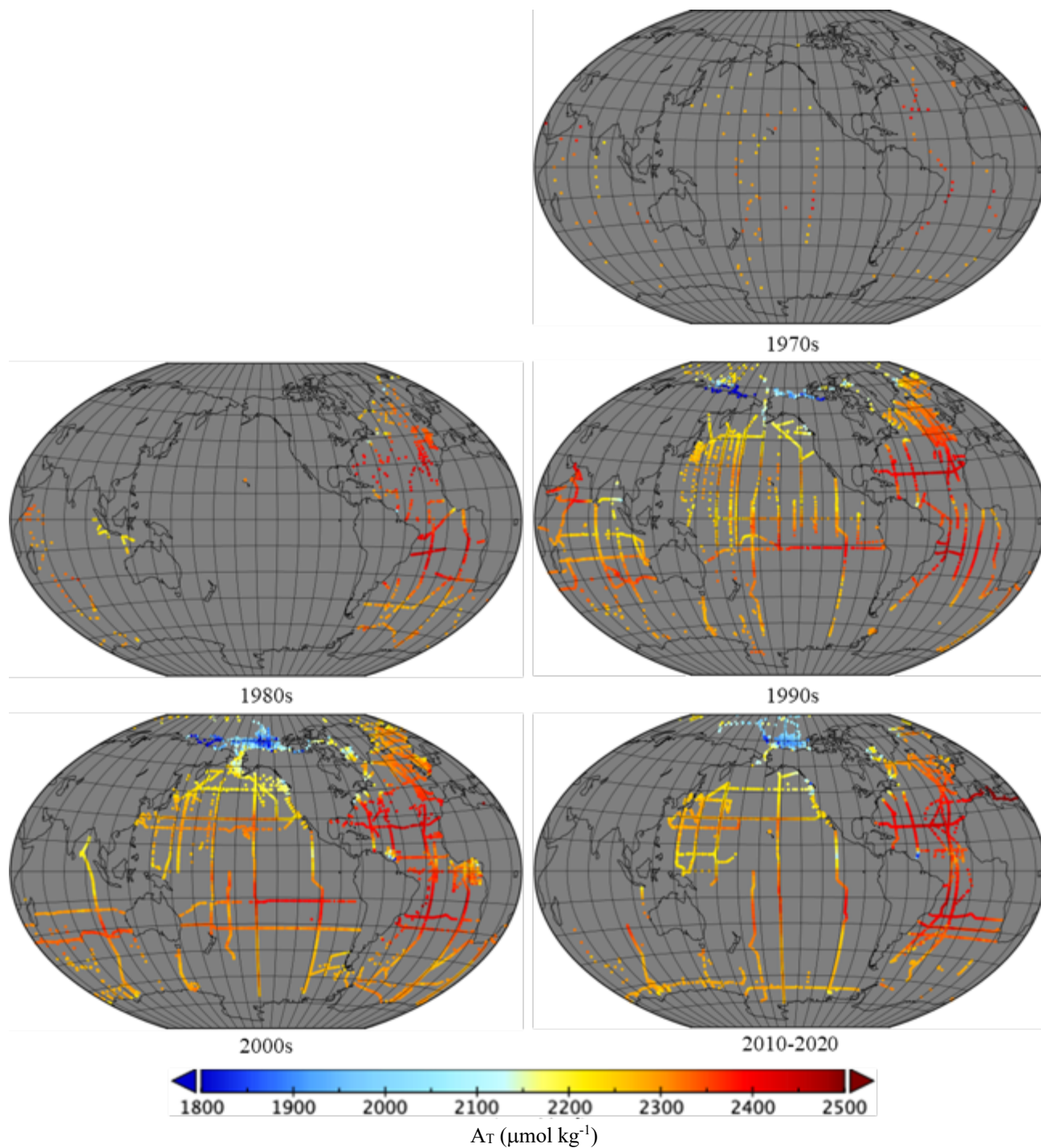
835 Figure 12. Mean A_T ( \mu\text{mol kg}^{-1} ) divided into decades: 128 ROIs in the 1970s; 707 in the 1980s; 3923 in the 1990s; 5196 in the 2000s; 3641 from 2010 to 2020.
