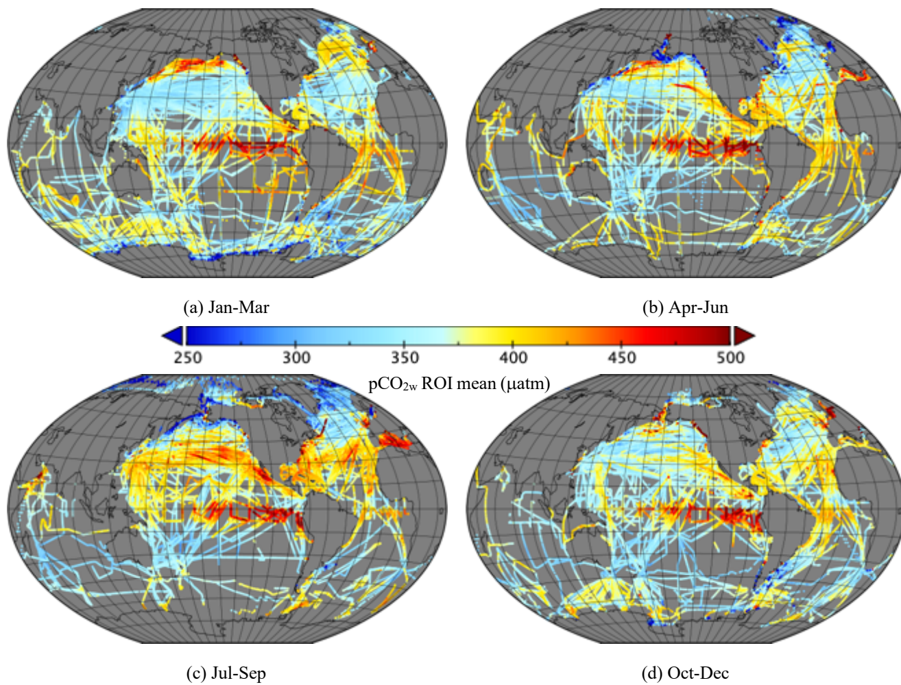
Figure 7. Mean pCO 2w (µatm) divided into seasons. (a) January – March (70,658 ROIs); (b) April – June (67,631 ROIs); (c) July – September (69,083 ROIs); (d) October – December (65,381 ROIs).
