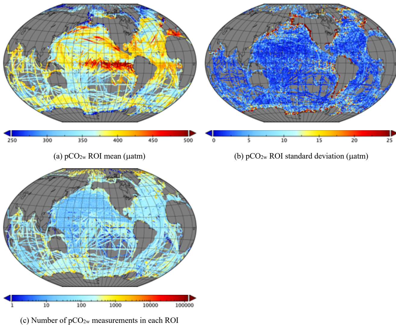
805 Figure 3. Statistics of pCO 2w in each ROI over the whole database (272,753 ROIs). (a) ROI mean, (b) ROI Standard deviation, and (c) number of measurements in each ROI.
