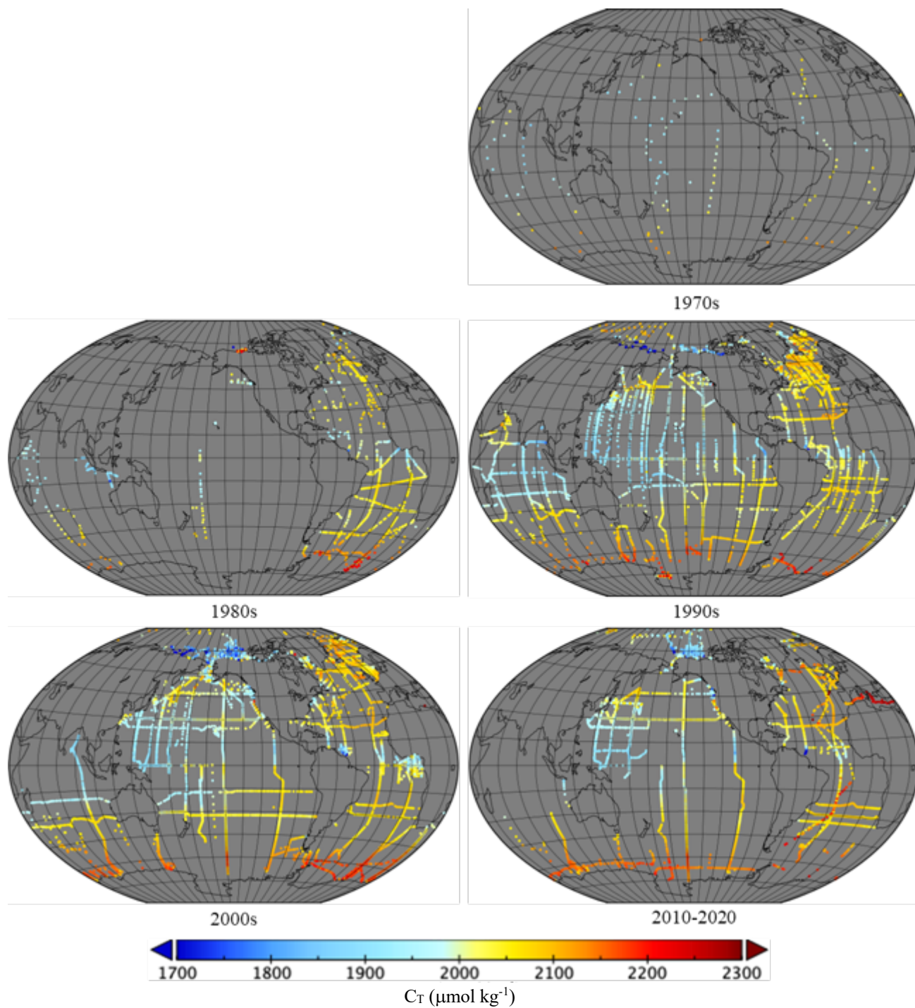
840 Figure 13. Mean C_T ( \mu\text{mol kg}^{-1} ) divided into decades: 123 ROIs in the 1970s; 971 in the 1980s; 4613 in the 1990s; 5672 in the 2000s; 3662 from 2010 to 2020.
