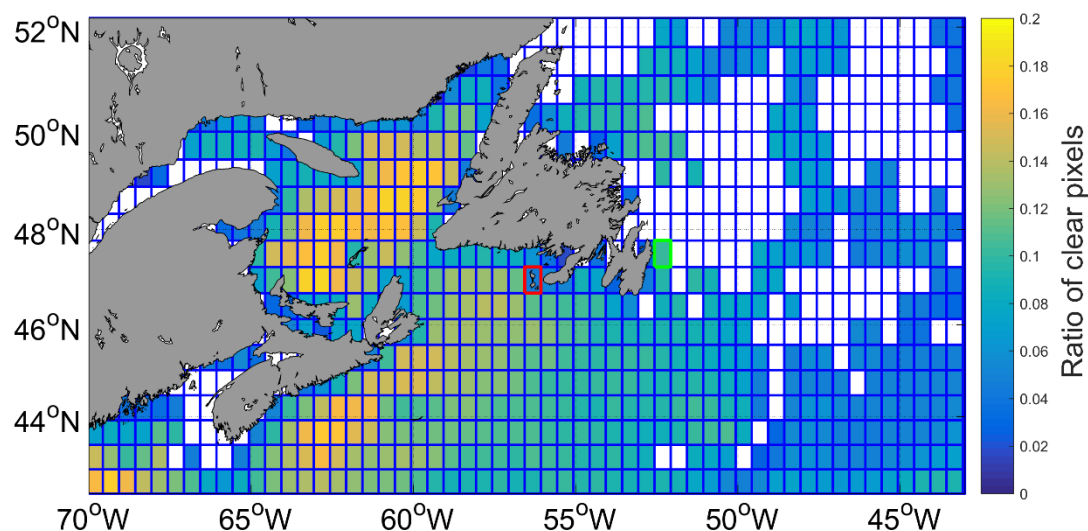
Fig. A1. Map displaying average ratio (theoretical maximum=1) of clear pixels (quality >=5) used in each grid box (33' latitude and 30' longitude including 13x12=156 pixels) for Fig. 8 August satellite SST spatial analysis (Pathfinder V5.3 dataset from Saha et al. (2018)). White boxes included at least one missing year over the 37-year time series. The green-sided rectangle circles the box used to extract August satellite SST time series from around station 27 (Fig. A2). The red-sided rectangle circles the box used to extract August satellite SST time series from Saint-Pierre and Miquelon coastal water used in Fig. 6 and 7 analyses. Due to a stroboscopic effect, 4 boxes lines contain 14x12=168 pixels. The entire domain spans 60x23 boxes.
