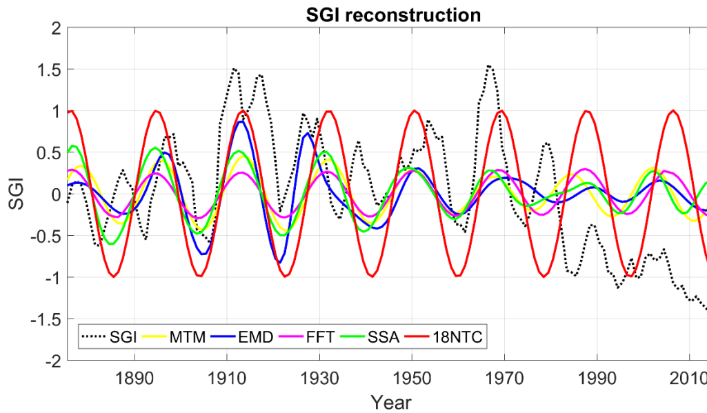
Fig. 4. Master chronology time series reconstructions at an 18.6-year period over time. Yellow line: Multi-taper method (MTM) reconstruction from harmonic components significant at the 95% confidence interval. Blue line: third intrinsic mode function (IMF) from an empirical decomposition method (EMD) analysis. Magenta line: inverse fast Fourier transform (FFT) reconstruction of the 18.6-year period. Green line: singular spectrum analysis (SSA) ( M = 45 ) reconstruction from the sum of reconstructed components (RCs) 5 and 6. Red line: astronomical 18.6-year nodal tidal cycle (18NTC) (arbitrary amplitude). Black dotted line: standardized growth index (SGI) 5-year running average.
