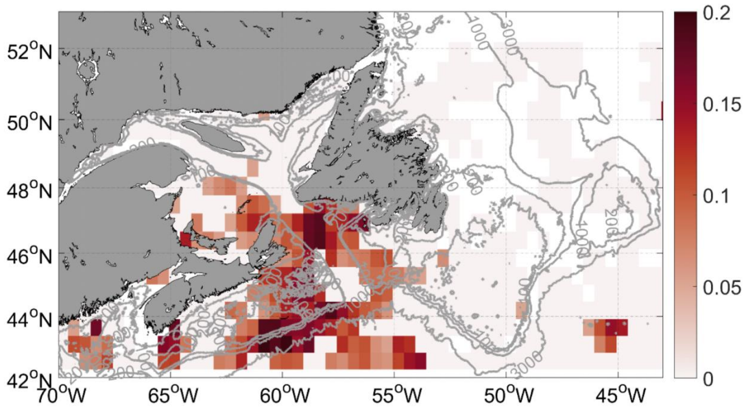
Fig. 8. Ratio of satellite SST variance (color scale on the right) for Least Square Method fitted SST series extracted from each 33' latitude and 30' longitude boxes whose phases are in opposition to the 18.6-year nodal tidal cycle (18NTC series) by \pm 1 year. Gray lines represent 3000, 1000, 200 and 100 m isobaths.
