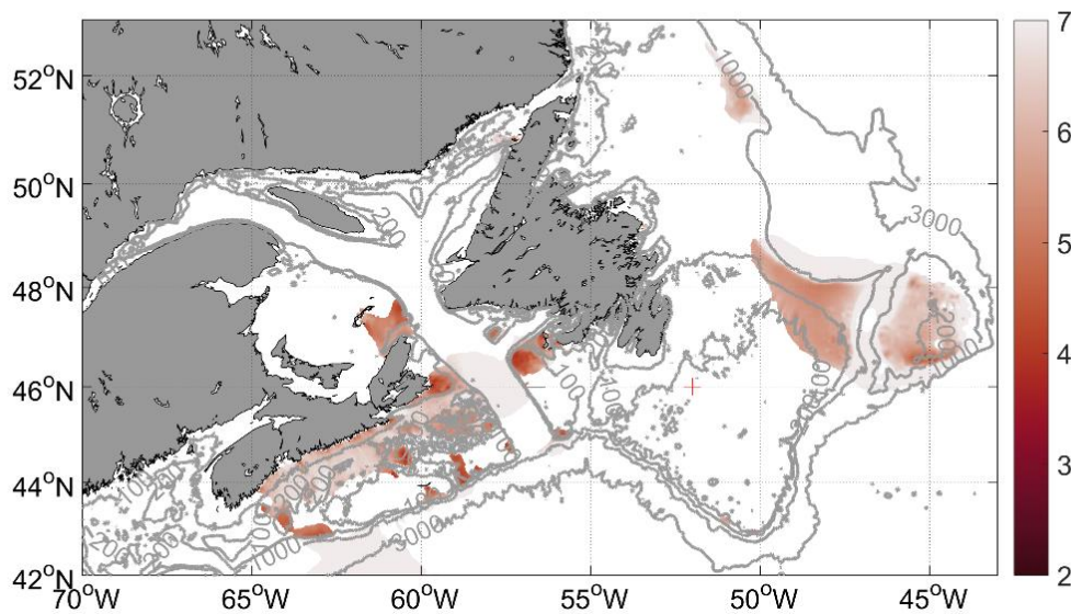
Fig. 9. Simpson-Hunter parameter (colored logarithmic scale displayed on the right) calculated over a duration of a month from diurnal currents obtained from Bezaud et al. (2020) model simulations ran from 2014/01/01 to 2014/03/16 with a spin-up of 0.5 months and shaded when its value is lower than the Simpson-Hunter parameter calculated for semi-diurnal currents obtained from the same model simulations. Gray lines represent 3000, 1000, 200 and 100 m isobaths.
