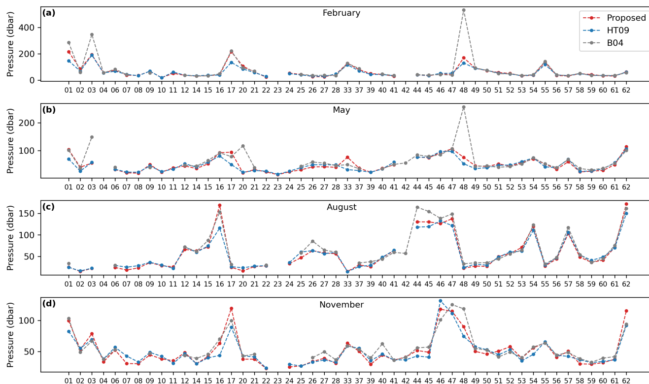
Figure 6. Comparison of methodologies to locate the MLD in (a) February, (b) May, (c) August and (d) November.
