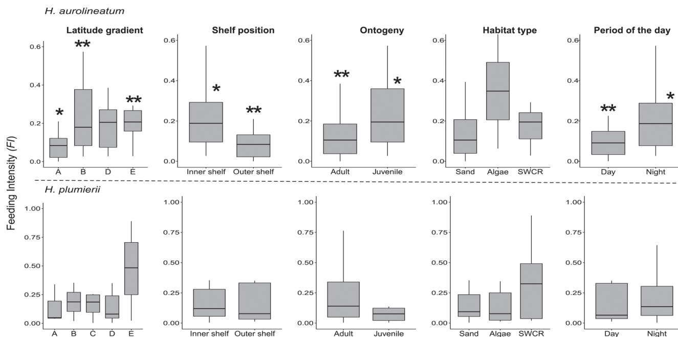
FIGURE 2 | Feeding intensity indicator ( F_i ) of Haemulon aurolineatum and H. plumierii in different habitats, latitude gradient, shelf position, ontogeny and period of the day. The black horizontal line and box represent the median value and the interquartile range, while the vertical lines represent the upper and lower limits. Outliers were not included in the plot. Different symbols (* and **) represent significant difference.
