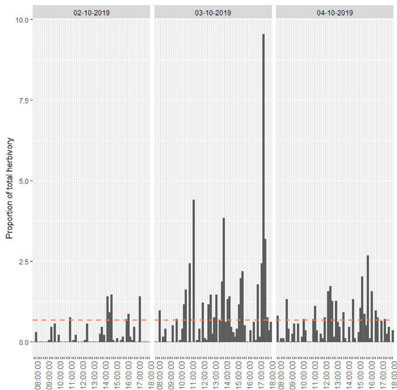
Figure 5. Variation of the fish grazing activity based on the proportion of total grazing realized per sequence (1min40s) throughout the three sampling days with the four 1m 2 -drops pooled. Red dotted line shows the proportion of herbivory per sequence expected if the herbivory is temporally uniform.
