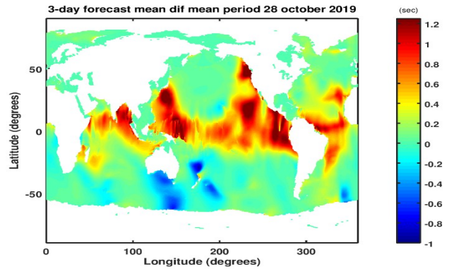
Figure 3 : Average of 3-hourly difference of mean wave period (in seconds) between run A after 3-day forecast and run C during 28 October 2019. Positive and negative values stand for underestimation and overestimation of model mean wave period.
