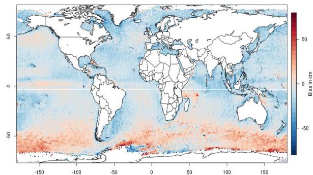
Figure 2 : Same as Figure 1, but for run C.
