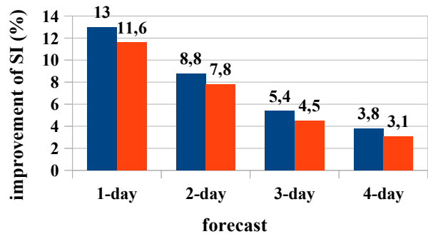
Figure 3 : Reduction of scatter index (in %) of SWH in the forecast period compared to control run C. Blue and red bars stand for run A and B, respectively.
