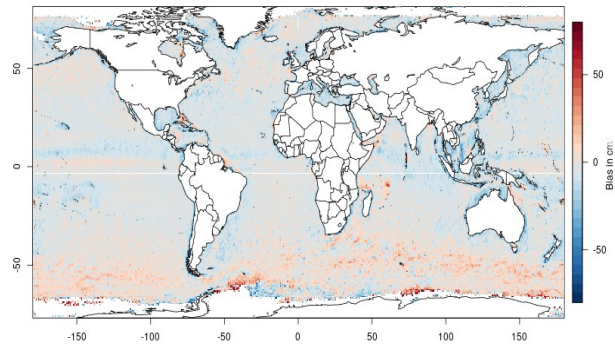
Figure 1 : bias map (in centimeters) of SWH from run A during Austral winter (May-August 2020). The comparison has been performed with altimeters Jason-3, Saral and Sentinel-3.
