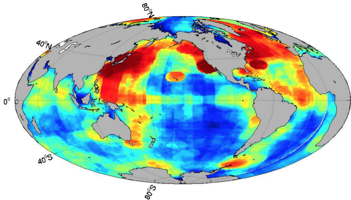
temporal data coverage, 1958-2015 (%)
