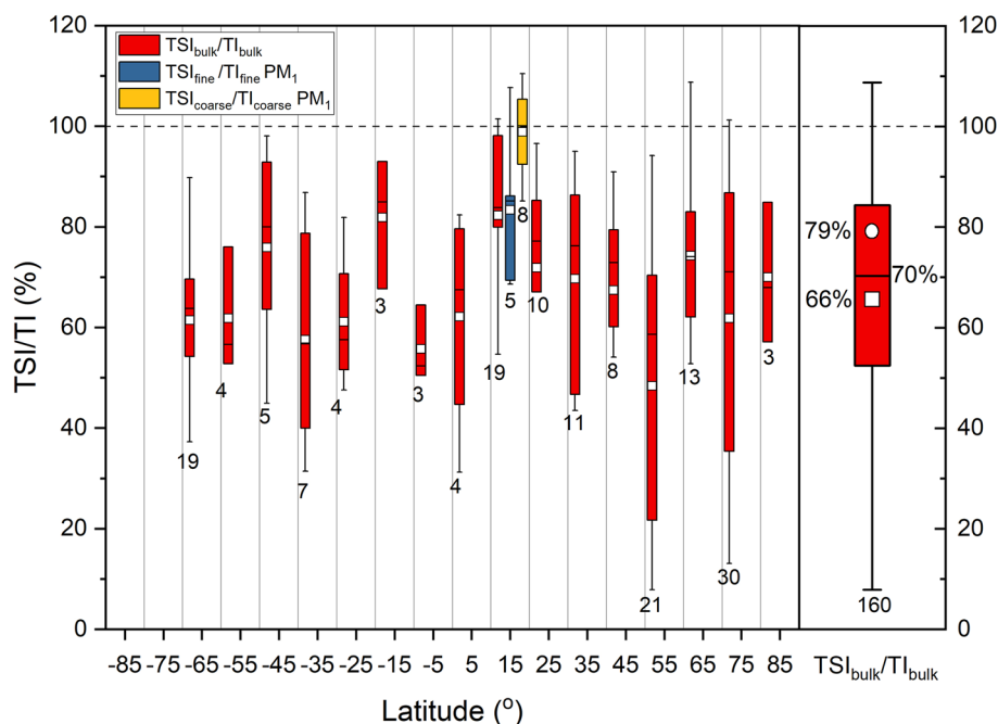
Figure 2. Left panel: latitudinal dependence of the TSI to TI ratio in bulk aerosol (red boxes), in the fine PM 1 fraction (blue), and the coarse fraction (yellow). Right panel: statistics of the TSI/TI ratio in bulk aerosol. The box and whiskers plot statistics are as follows: interquartile range (box), 1.5 × interquartile range (whiskers), median (horizontal line), mean (square), and outliers (diamonds). The circle indicates that the TSI fraction derived from the slope of the TI versus TSI error-weighted linear fit (Gómez Martín et al., 2021). The number of samples is indicated below the boxes.
