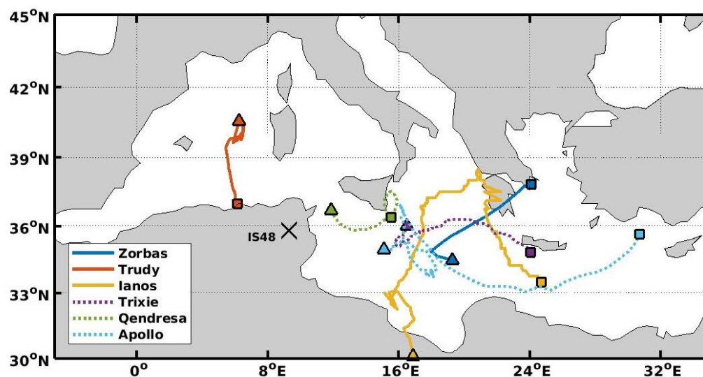
Figure 1. Trajectories of the medicanes considered in the study and presented in Section 2.6. Markers indicate the beginning of the recorded trajectory (triangle) as well as the end of it (square). The black cross shows the location of the infrasound station IS48 in Tunisia. The trajectories drawn with a solid (resp. dotted) line indicate medicanes for which significant infrasound detections could (resp. not) be observed at the station, at least in one of both frequency ranges considered in the paper.
