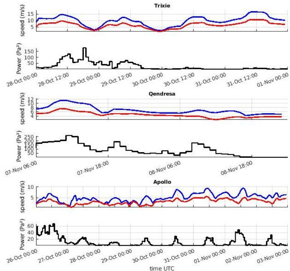
Figure 12. Time-series of ERA5 10-m wind (red line) and gusts (blue) ( m/s ) at IS48 during Trixie (top), Qendresa (middle), and Apollo (bottom), along with acoustic power integrated between 0.01 and 0.1 Hz (black line), as presented in Figure 3b and c for Trudy, for instance.
