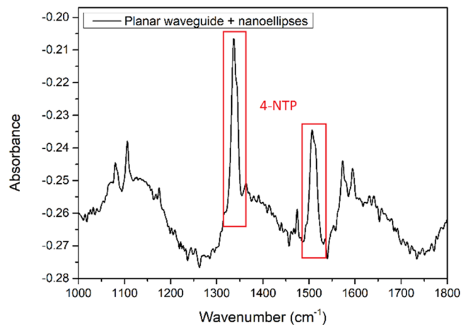
Figure 12. Absorbance spectra of 4-NTP on a chalcogenide waveguide coated with gold nanoparticle substrates.
