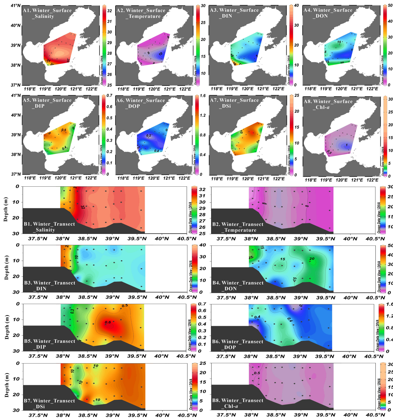
FIGURE 5 Distribution of salinity (psu), temperature ( ^{\circ}\text{C} ), DIN concentration ( \mu\text{mol}\cdot\text{L}^{-1} ), DON concentration ( \mu\text{mol}\cdot\text{L}^{-1} ), DIP concentration ( \mu\text{mol}\cdot\text{L}^{-1} ), DOP concentration ( \mu\text{mol}\cdot\text{L}^{-1} ), DSi concentration ( \mu\text{mol}\cdot\text{L}^{-1} ) and Chl-a concentration ( \mu\text{g}\cdot\text{L}^{-1} ) at surface layer (A1-A8) and Northeast-Southwest transect (B1-B8) in winter.
