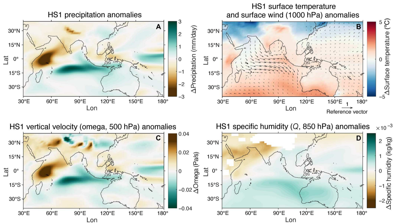
Fig. 3. Simulated climate anomalies over the tropical IO. Changes in (A) precipitation, (B) surface temperature and surface wind at 1000-hPa level, (C) vertical velocity ( \omega ) at 500-hPa level, and (D) specific humidity ( Q ) at 850-hPa level during HS1 relative to BA in response to MWF in iTRACE. The HS1 coastlines (black outline) correspond to a 120-m drop in sea level.
