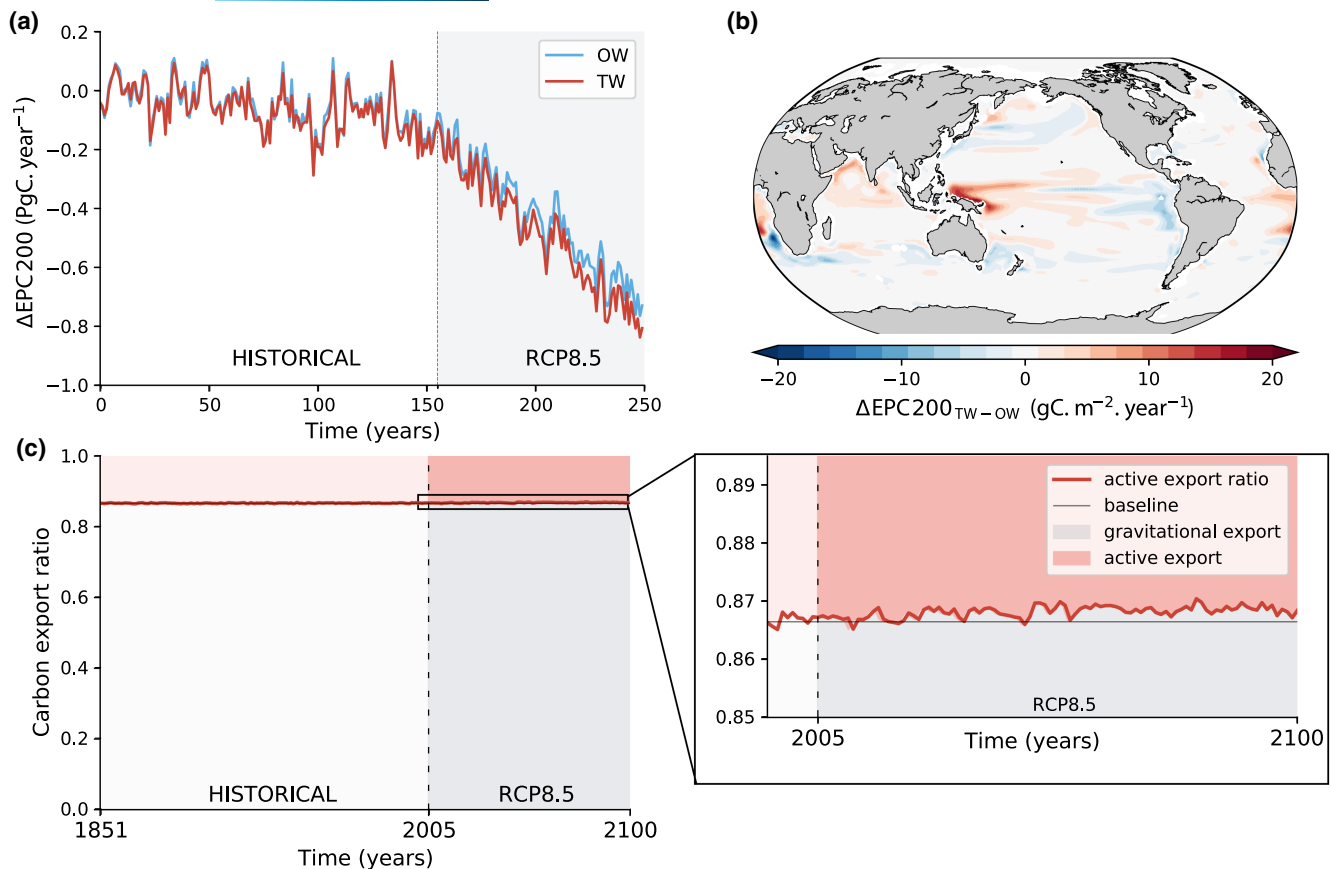
FIGURE 2 Influence of climate change on carbon export in the OW and TW coupling schemes. (a) Time series of the mean carbon export anomaly ( \text{PgC} per year) at 200m depth. The anomaly is computed relative to the averaged carbon export over the first 20 years of the historical period (1851–1870). The blue curve corresponds to the OW simulation and the red one to the TW simulation. (b) Map of the difference in export anomaly between the TW and OW simulations ( \text{TW}-\text{OW} , \text{PgC} \cdot \text{year}^{-1} ), and (c) detailed analysis of the export at 200m for the TW simulation, the grey and red areas represent the proportion of passive and active export, respectively, to the total carbon export. The red line represents the distinction between passive and active export in time, called the active export ratio here. The grey line, named baseline, is the averaged contribution of passive versus active export during the historical time period. A regional analysis of the export can be found in the Supplementary Material (Figure S2). OW, one-way; TW, two-way.
