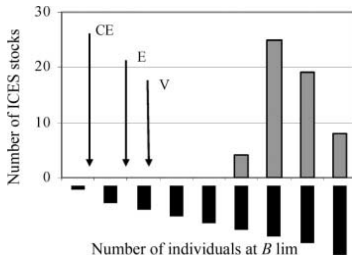
Figure 3.4: Histogram of the number of (ICES) stocks with B_{lim} converted into approximate numbers of N_{lim} (x-axis in arbitrary bins). V, Vulnerable; E, Endangered; CE, Critically Endangered (following Rice & Legacé 2007).
