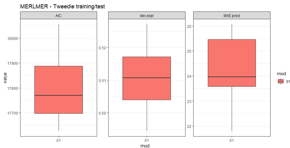
Figure 4.1.2.29. Train/test results: AIC, explained deviance and MAE.
