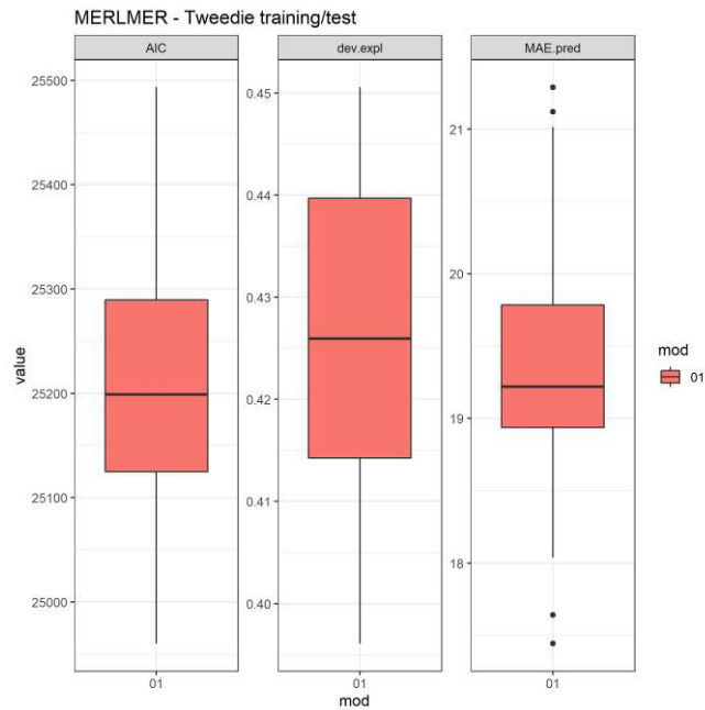
Figure 4.1.2.5. European hake GSAs 18–19–20. Train/test results: AIC, explained deviance and MAE.
