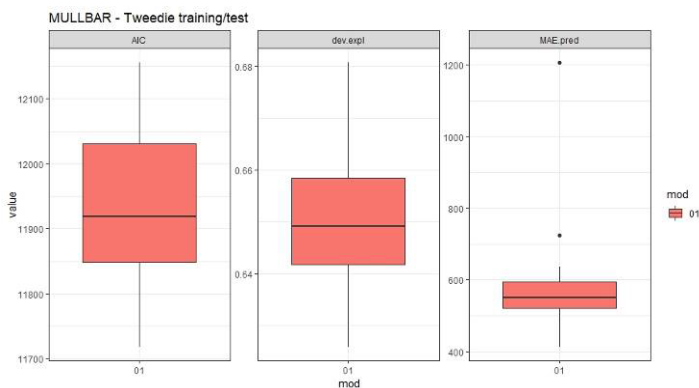
Figure 4.1.2.17 Train/test results: AIC, explained deviance and MAE.
