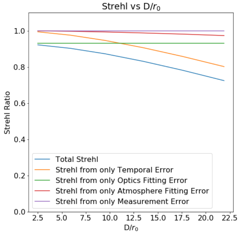
Fig 6 Estimated Strehl Ratio for each of the D/r_0 values simulated in CACTI. The total Strehl value is the highest estimated closed-loop Strehl value achievable on CACTI when considering all of the terms in the error budget. The other lines are plots of the expected Strehl values when only considering a single term from the error budget.
