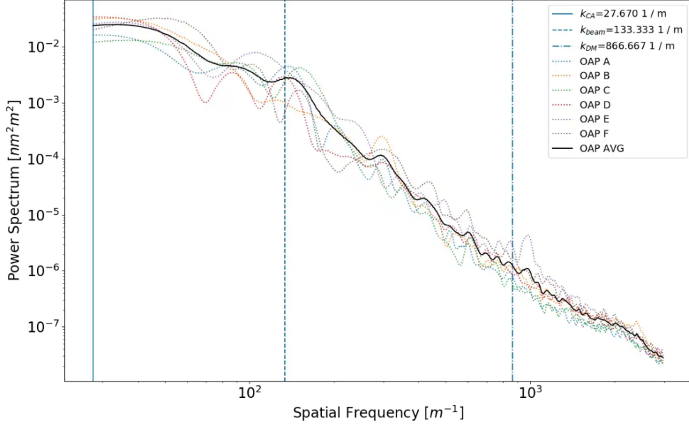
Fig 4 Power spectrum estimate versus spatial frequency of the OAP mirrors. The solid black line is the average PSD estimate for all OAPs. Overlaid on this plot are vertical blue lines representing the lower spatial frequency boundary used to calculate the root-mean-square (RMS) surface error for different parameters such as beam size and DM correction. These boundaries can be read as all spatial frequencies to the right of each line are included in the RMS calculation. The first line ( k_{CA} ) represents the 75% clear aperture of the OAP mirror. The middle line ( k_{beam} ) represents the lower spatial frequency limit from our 7.5 mm beam diameter. The final line ( k_{DM} ) represents the lower spatial frequency limit corrected by the DM for the 7.5 mm beam diameter in our PSF sharpening process.
