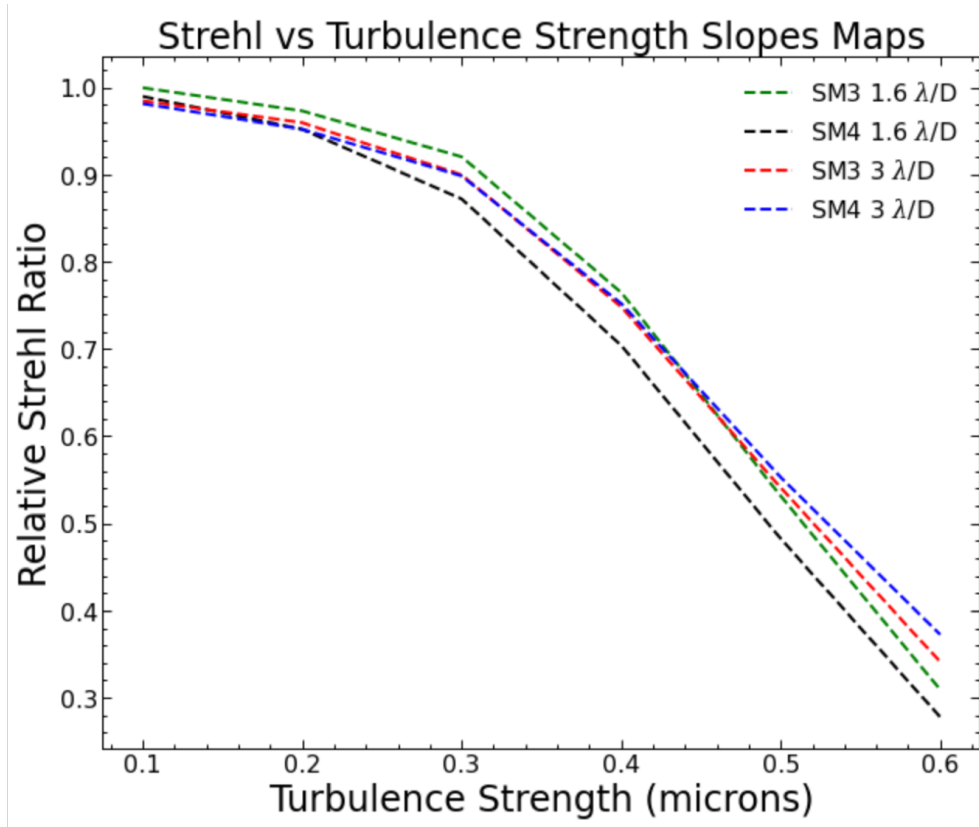
Fig 14 Relative Strehl ratio versus turbulence strength for the 3PWFS and 4PWFS using the Slopes Maps signal processing method. The performance of each wavefront sensor across all modulations radii and turbulence strengths are comparable.
