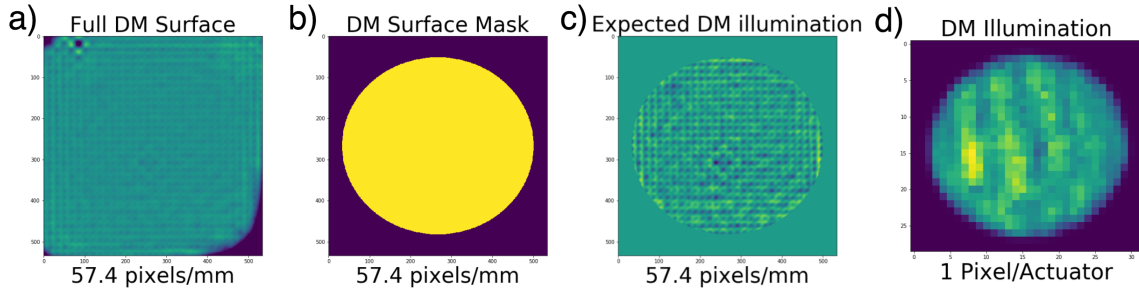
Fig 5 A. Surface map of the flattened DM measured by an interferometer. B. The estimated DM surface illumination pattern by our optical design. C. The surface map of the flattened DM masked by the DM surface mask given in B). D. The calculated DM illumination pattern from our calibration procedure.
