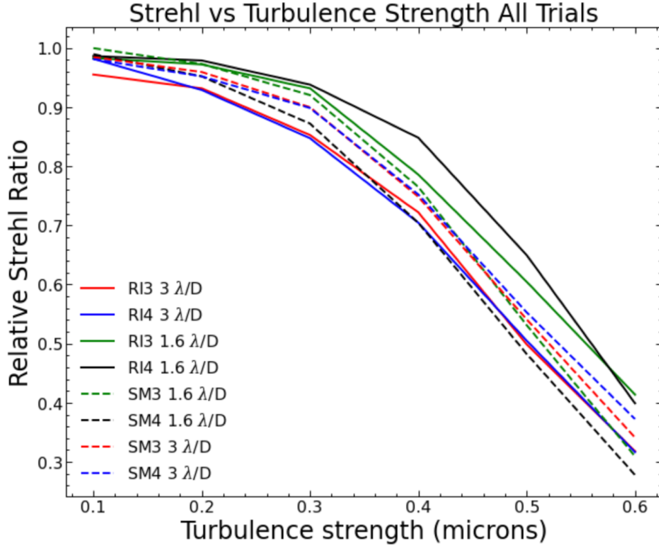
Fig 15 Summary of all results. Best performance was achieved using the 4PWFS at 1.6 \lambda/D modulation using RI. However, this trial had the highest modal gains set, suggesting that this performance difference is not real, and that the modal gain for the other trials was set too low.
