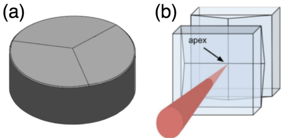
Fig 7 Drawings of the pyramid optics in CACTI. A. The 3PWFS pyramid is a single prism made from fused silica glass. The 4PWFS pyramid is two crossed roof prisms. This pyramid is a copy of the pyramid used by SCEXAO. This drawing is Figure 2. from Jovanovic et al. 26
