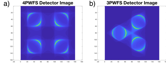
Fig 1 Simulated PWFS detector images under no modulation for the 4PWFS (a) and the 3PWFS (b).
