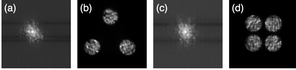
Fig 11 A. Time-averaged science camera image of the 3PWFS closed-loop PSF in log scale. B. Turbulence streaming across the 3PWFS pupils. C. Time-averaged science camera image of the 3PWFS closed-loop PSF in log scale. D. Turbulence streaming across the 4PWFS pupils.
