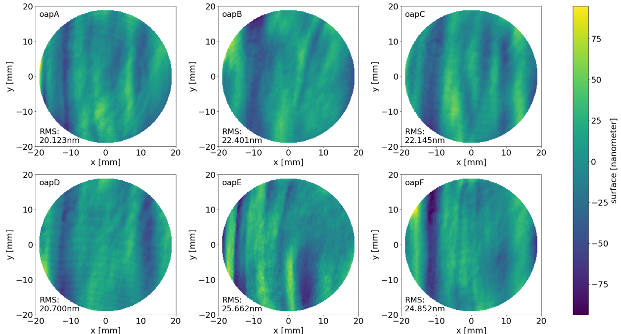
Fig 3 Surface measurements of the OAP mirrors in CACTI. In color scale is the surface error in nanometers. All mirrors were cored from the same parent and specified at \lambda/10 surface quality.
