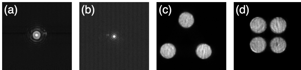
Fig 10 Signals from CACTI in response to the optimized flat wavefront. A. The PSF on the science camera. B. The optimized PSF on the focal plane of the PWFS tips. C. The 3PWFS pupils on Camzyla at 5 \lambda/D modulation. D. The 4PWFS pupils on Cam4p at 5 \lambda/D modulation.
