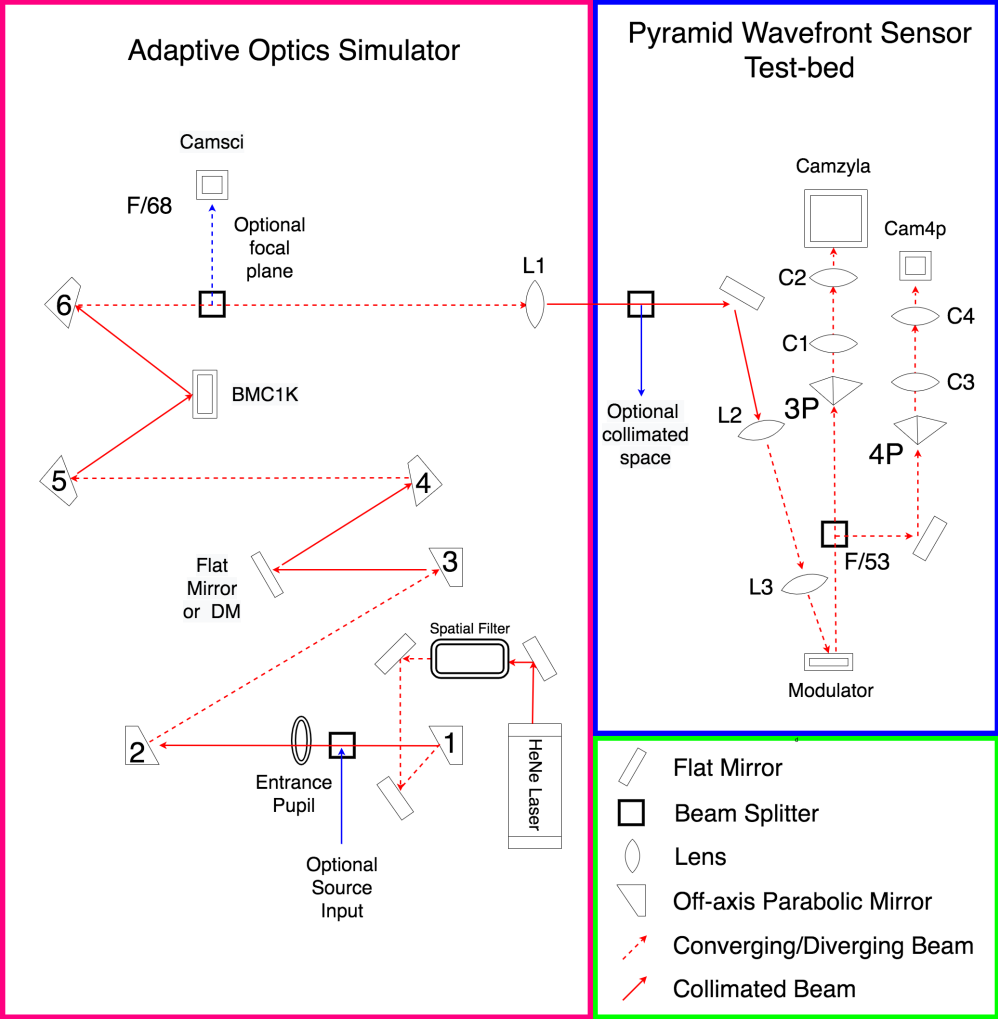
Fig 2 In the current configuration CACTI consists of an Adaptive Optics Simulator and the PWFS testbed. Beam-splitters are used in CACTI to provide access to focal planes, collimated spaces, and additional sources. In the current configuration light is relayed through the AO simulator onto the 1024 actuator Boston Micromachine 1K (BMC1K) DM OAP mirrors. The light is then passed to the PWFS testbed which includes a modulation mirror, a 4PWFS and a 3PWFS. The F-number on the pyramid tip is F/53, and the F-number on camsci is 68.
