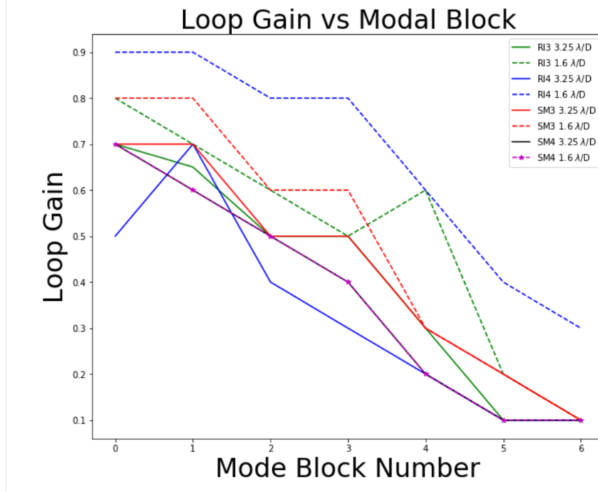
Fig 12 Loop gain value optimized for the PWFS configuration plotted against the corresponding modal block number in CACTO. The modal gains for SM3 3.25 \lambda/D and SM4 1.6 \lambda/D were the same. To differentiate we have over plotted the SM4 1.6 \lambda/D line in magenta dashes and stars. The gain was optimized at low turbulence, and the same values were used for all turbulence strengths.
