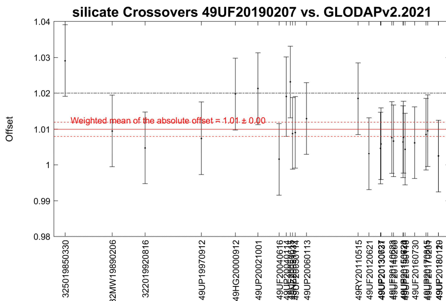
375 Figure 4. Example summary figure, for silicate crossovers for 49UF20190207 versus the cruises in GLODAPv2.2021 (with cruise EXPCODE listed on the x axis sorted according to year the cruise was conducted). The black dots and vertical error bars show the weighted mean offset and standard deviation for each crossover (as a ratio). The weighted mean and standard deviation of all these offsets are shown in the red lines and are 1.01 \pm 0.00 . The dashed black lines are the reference line for a \pm 2\% offset.
