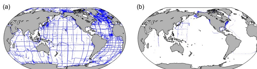
190 Figure 1. Location of stations in (a) GLODAPv2.2021 and for (b) the new data added in this update.
