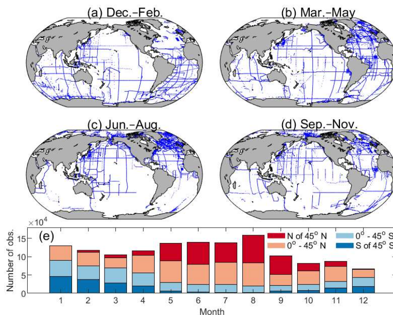
670 Figure 10. Distribution of data in GLODAPv2.2022 in (a) December–February, (b) March–May, (c) June–August, and (d) September– 675 November, as well as (e) number of observations for each month in four latitude bands.
