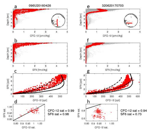
460 Figure 6. Example of plots used as basis for the SF 6 QC procedure. Shown are results for cruises 096U20160426 (left) and 320620170703 (right). a, e) CFC-12 versus pressure for the specific cruise (red), together with all data from the corresponding GLODAP region (Pacific in this case, grey). b, f) Same as upper row, but for SF 6 . c, g) CFC-12 versus SF 6 (red dots), here the measured contents have been converted into atmospheric mixing ratios. Solid black line: atmospheric time history of CFC-12 vs. that of SF 6 . Dotted lines: CFC-12 vs. SF 6 derived from the TTD method for two different sets of TTD parameters. d, h) CFC-12 vs. SF 6 saturation for the surface layer (P < 20 dbar), where the numbers give the mean saturation.
