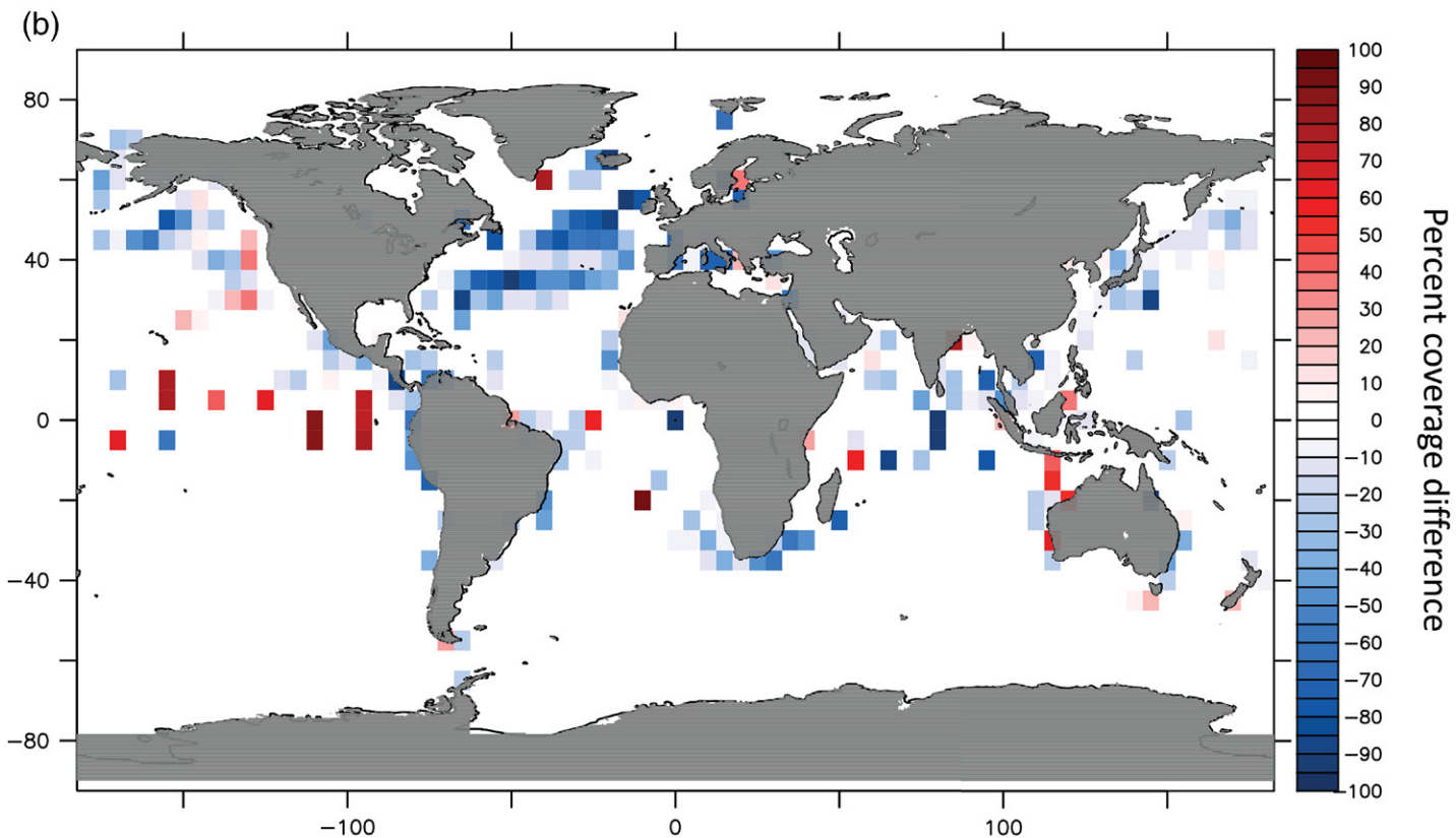
Air temperature coverage difference between Apr-Jun 2021 and 2019
