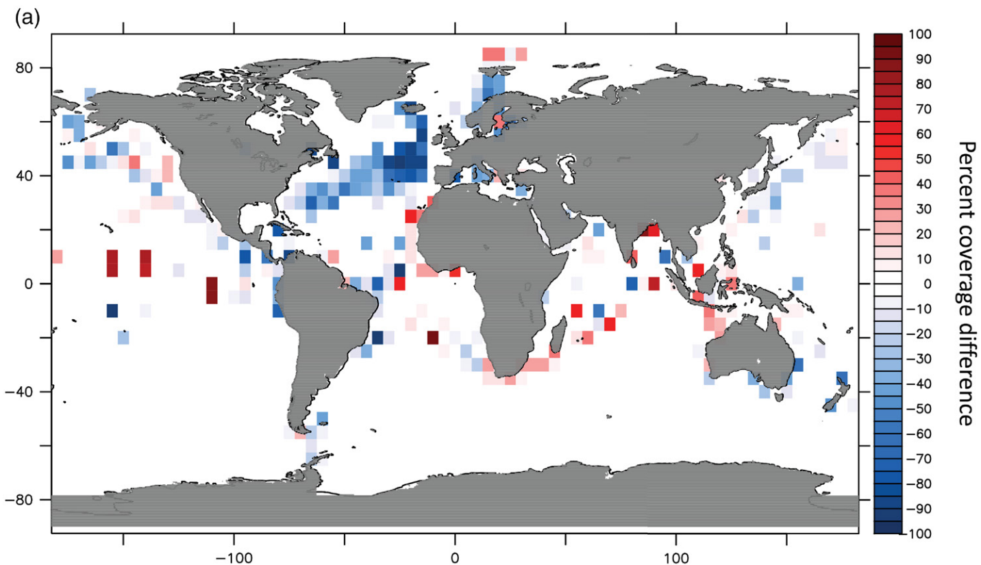
Air temperature coverage difference between Apr-Jun 2020 and 2019
