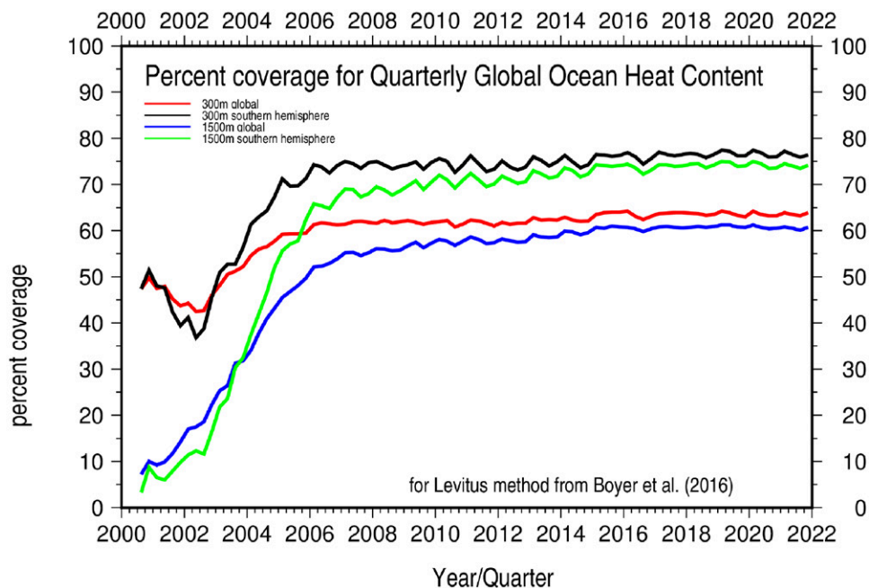
Fig. 15. Percent coverage of subsurface temperature data at 300 and 1,500 m depth globally and for the Southern Hemisphere by season (3-month period) during 2000–21 for the calculation of ocean heat content, calculated as the fraction of 1^\circ \times 1^\circ lon–lat grid boxes with at least three temperature measurements within 400 km of the gridbox center.
