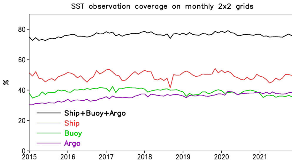
Fig. 14. Percent global coverage of monthly sea surface temperature (SST) measurements during January 2015–December 2021, calculated as the fraction of 2^\circ \times 2^\circ lon–lat grids with at least one SST report for the month.
