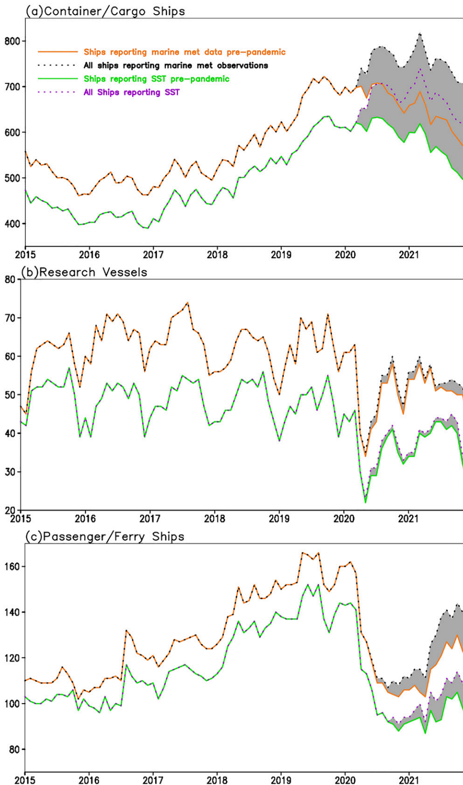
Fig. 2. Number of ships with independent WMO call sign numbers since 2015 in the ICOADS R3.0.2 near-real-time collection. (a) The container/cargo ships, (b) the research vessels/ships, and (c) passenger/ferry ships. The orange and black lines are for all ships, compared to the green and purple lines, which are for subsets of ships reporting SST measurements. The solid lines are for the number of ships that were reporting data pre-pandemic (defined as March 2020) and have continued since then, while the dashed lines are the total number of ships reporting data during the pandemic.
