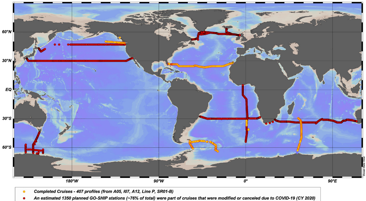
Fig. 4. Global Ocean Ship-Based Hydrographic Investigations Program (GO-SHIP) repeat hydrography cruises planned and/or completed in 2020. Cruises in red were planned but were subsequently ended prematurely, canceled, or delayed into the future. Orange dots show where profiles were measured in 2020 for completed and partially completed cruises.
