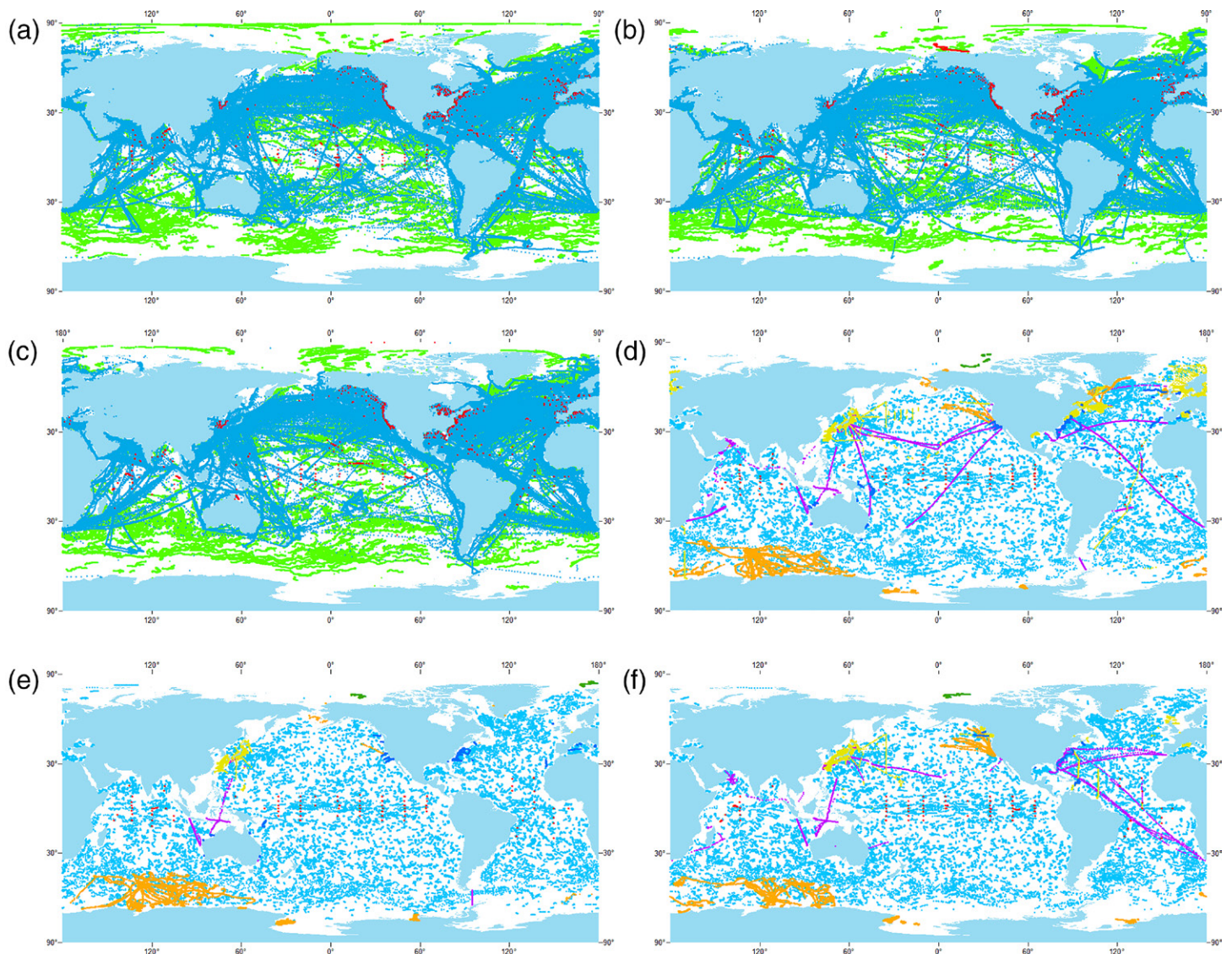
Fig. 1. Geographic distribution of marine meteorological and ocean surface observations from ships (blue), moored buoys (red), and drifting buoys (green) for April–June (a) 2019, (b) 2020, and (c) 2021. Subsurface observations (at any depth) from Argo floats (turquoise), expendable bathythermographs (purple), ship-based conductivity–temperature–depth (yellow), gliders (blue), tropical moored buoys (red), pinniped-mounted sensors (orange), and ice-tethered profilers (dark green) for April–June (d) 2019, (e) 2020, and (f) 2021. Note that surface observations from other platforms overlay drifting buoys (green) in (a)–(c) while subsurface observations overlay observations from Argo floats (turquoise) in (d)–(f). Drifting buoys and Argo floats are well represented, but not visible in all areas outside of marginal seas and high latitudes.
