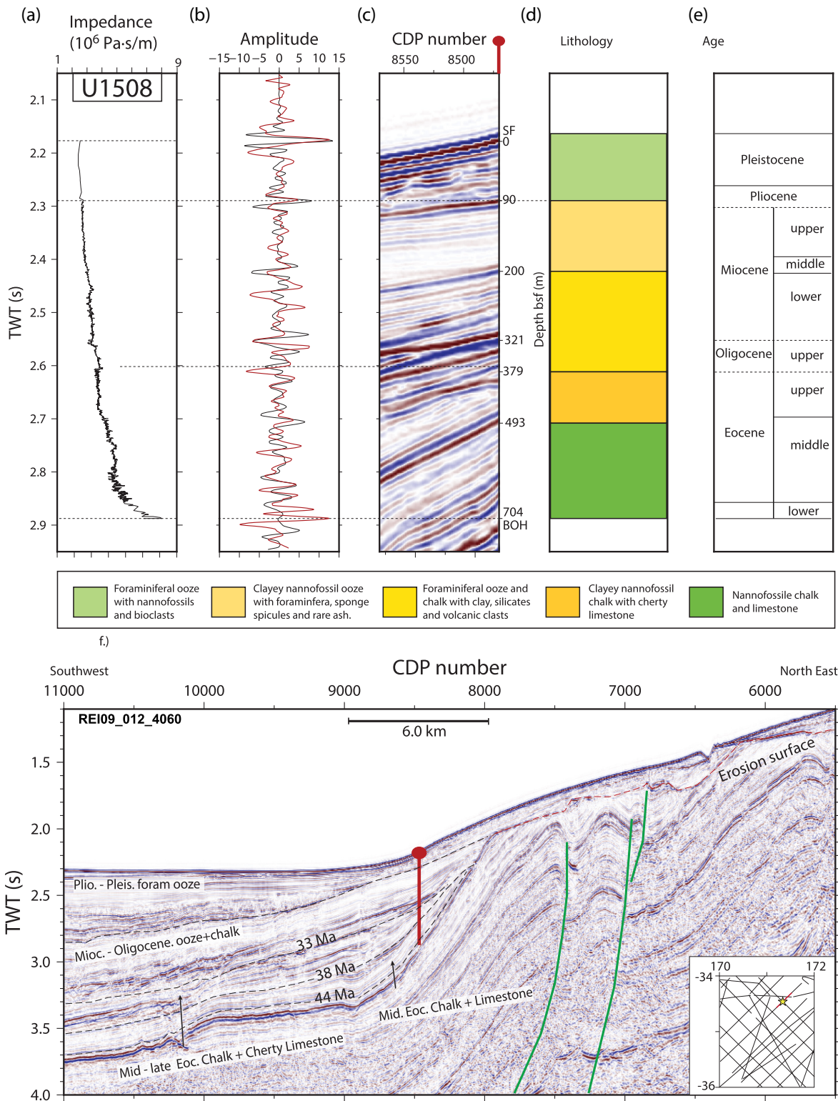
Figure 5. Borehole ties to seismic and timing of tectonic events at Site U1508. See the caption for Fig. 3 for further explanation. Green lines are fault traces.
