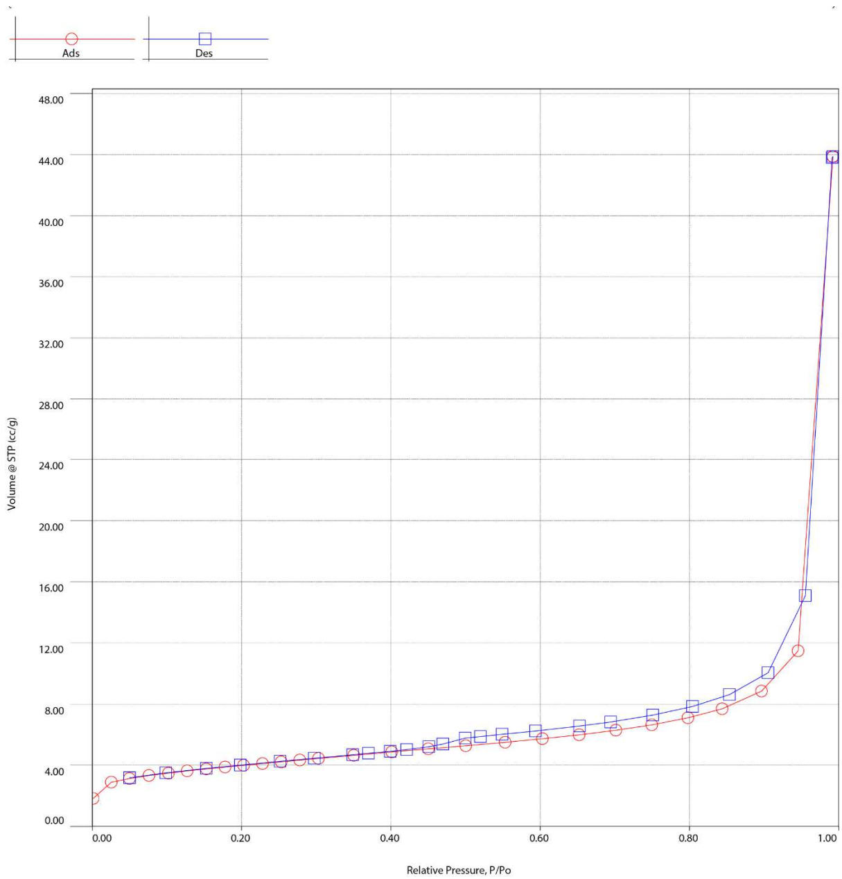
Supplementary Figure 1. Adsorption (red circles and curve) and desorption (blue squares and curve) isotherms for sample BV-VAR-08.
