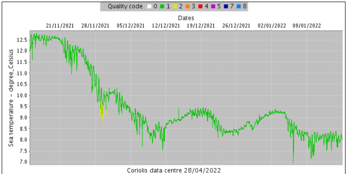
Figure S1: Temperature recorded from a Marel Carnot buoy (code 6200443) in front of Boulogne-sur-Mer between mid-November 2021 and mid-January 2022 (Coriolis data; Lefebvre, 2015).
