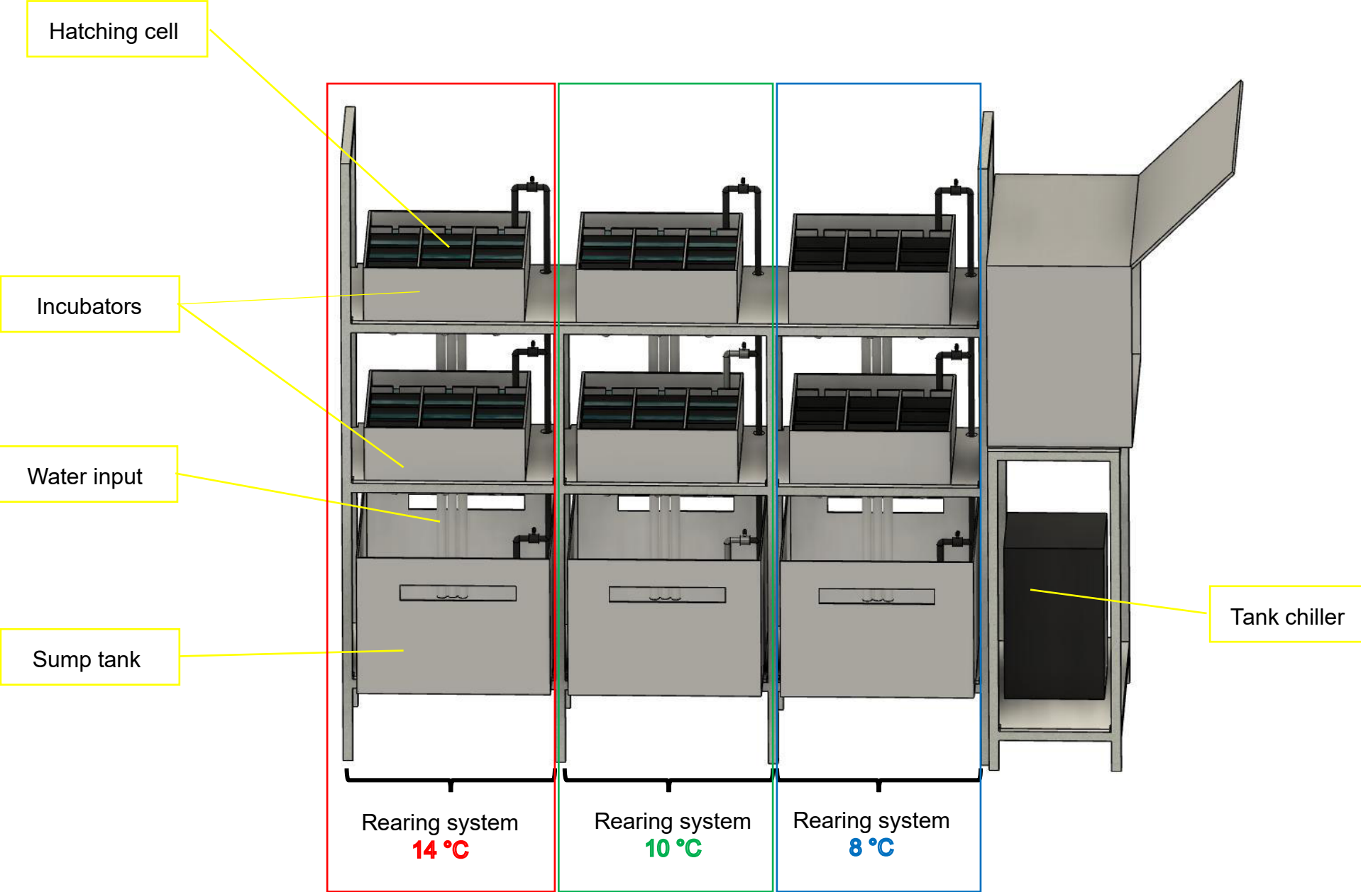
Figure S2: Experimental set-up
