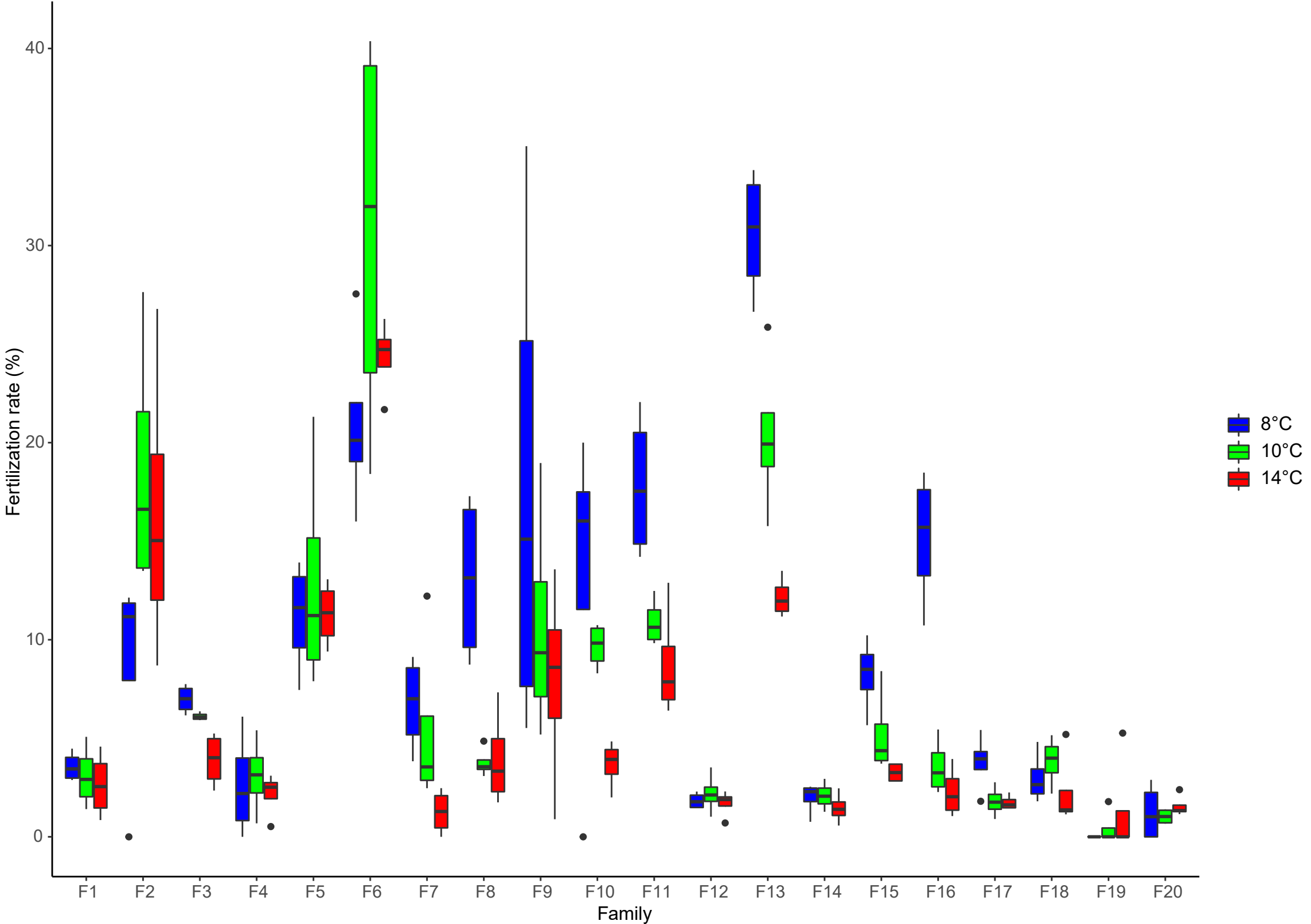
Figure S4: Boxplots of fertilization rate across the different families. Colors correspond to the three temperature scenarios: 8 °C (blue), 10 °C (green) and 14 °C (red).
