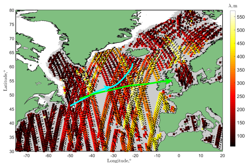
Figure 4. Measured \lambda_p (colored boxes) and \varphi_p after eliminating 180° ambiguity (black arrows) in “wave boxes” on two sides of the CFOSAT-SWIM track in Northern Atlantic during the period of 11 February 2020 00:00 UTC —16 February 2020 00:00 UTC, after applying ice and land masks. The green and cyan colored lines and arrows show the trajectory and direction of the ETC#1 and ETC#2, respectively.
