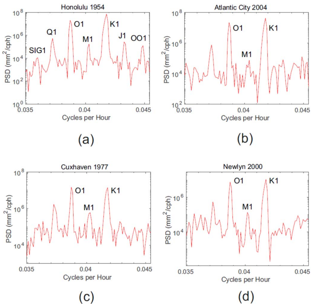
Figure 3. (a) Power spectral density (PSD) within the diurnal section of a spectrum of one year of sea level data from Honolulu, Hawaii showing the lines of the main diurnal tides. (b-d) The corresponding spectra from Atlantic City, Cuxhaven and Newlyn respectively.
