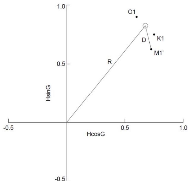
Figure 6. (a) An example of the positions of K1 and O1 in the complex plane, their mid-way position (open circle) and its amplitude (R), and the distance (D) between the measured M1' and the mid-way point.
