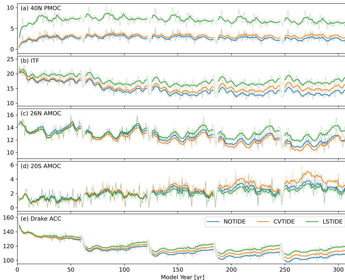
Figure 16. The time series of (a) 40^{\circ} N PMOC, (b) ITF, (c) 26^{\circ} N AMOC, (d) 20^{\circ} S AMOC, (e) ACC through the Drake Passage from the three sensitivity runs in all five cycles. The light and thin lines are original annual time series, and the dark and thick lines are five-year moving average results for each cycle. All vertical axes have the unit of Sv. Note that 26^{\circ} N AMOC and 20^{\circ} S AMOC denote the strength of AMOC upper cell and lower cell, respectively. The calculation of ITF and ACC flux through the transections in the Indonesian Archipelago and the Drake Passage applies the algorithm introduced in Sidorenko et al. (2020).
