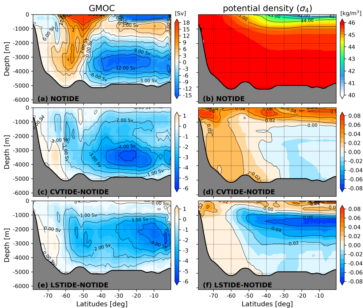
Figure 17. The GMOC and potential density with reference depth at 4000 m ( \sigma_4 ) in the southern hemisphere. The upper panels denote results in the control run, while the middle/lower panels denote the difference between CVTIDE/LSTIDE and NOTIDE. Note that the potential density in the figure is globally zonal averaged, with meridional bin set to 1^\circ .
