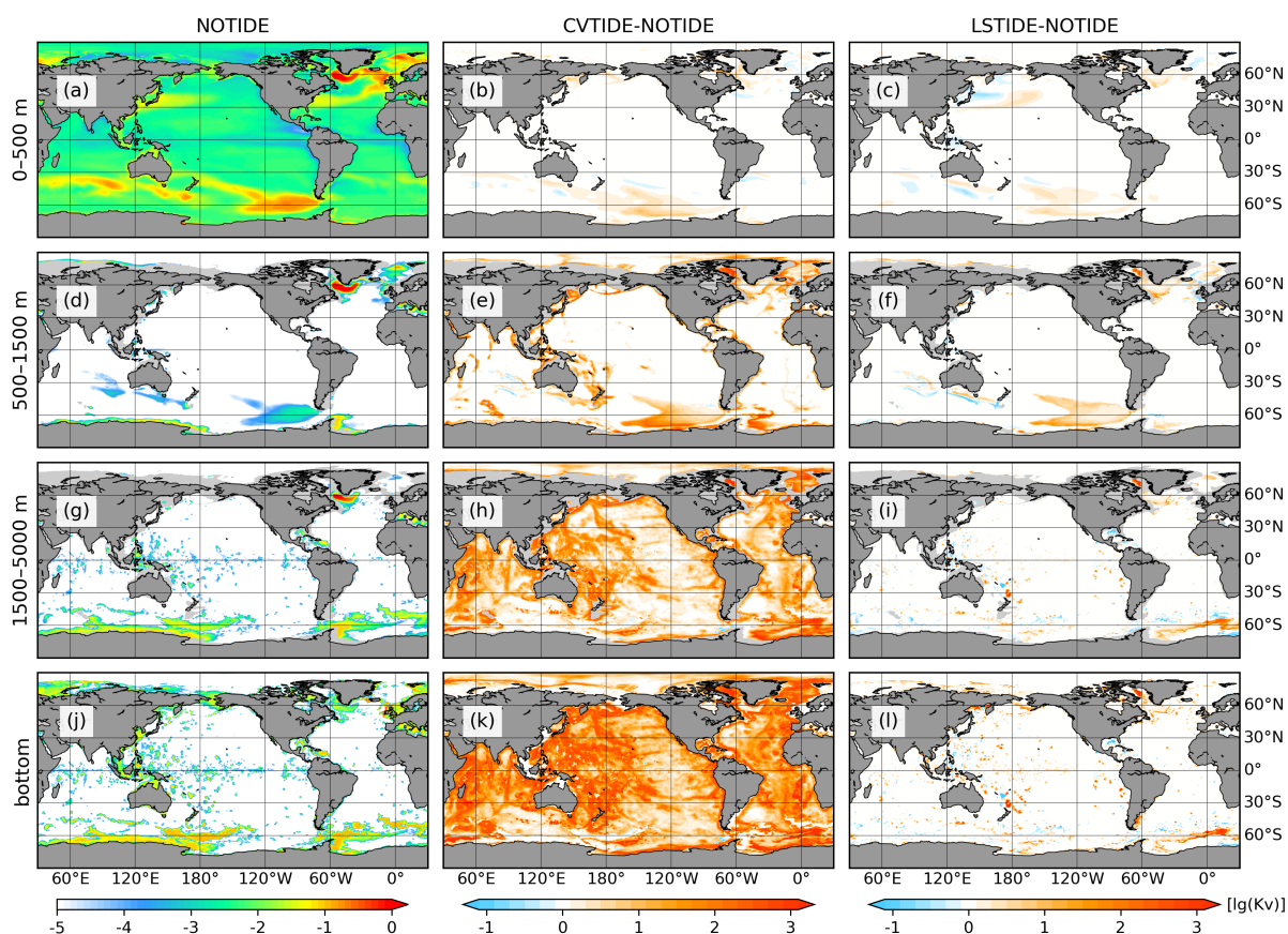
Figure 12. Depth averaged vertical diffusivity in the upper (0–500 m), intermediate (500–1500 m), deep (1500–5000 m) ocean, and the bottom layer of the ocean. The left column shows vertical diffusivity in the control run, while the middle/right column shows the difference between CVTIDE/LSTIDE and NOTIDE. Note that vertical diffusivity is shown in a decimal logarithm scale, and the middle/right column shows the difference of scaled vertical diffusivity.
