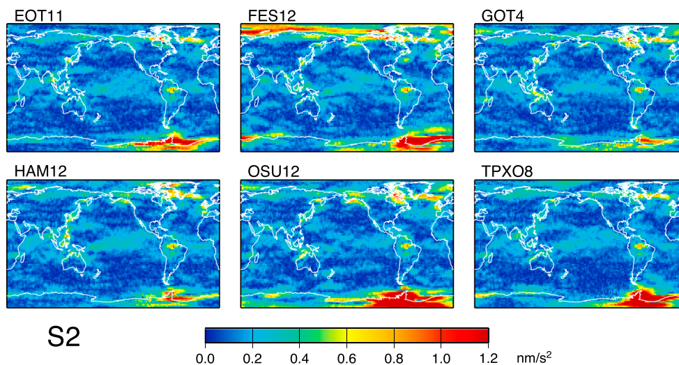
Figure 11. As in Figure 8 but for the S 2 frequency. The overall inflation of background noise stems from a multitude of possible β'-like errors in both GRACE data and in the ocean tide models themselves. Some signals, however, stem from inadequate modeling of hydrology, such as the small anomalies evident in the Amazon basin which may exist at the 160 day S 2 alias period for GRACE.
