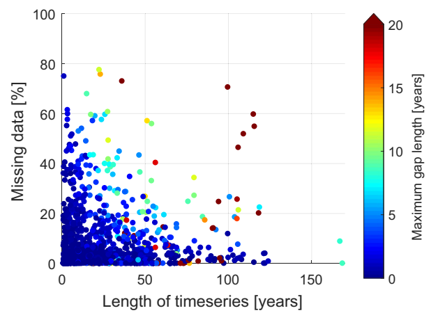
FIGURE 5 Percentage of missing data plotted against the time series length. The maximum gap length is colour coded. The plot shows the records after the removal of flagged data at each end of their time series
