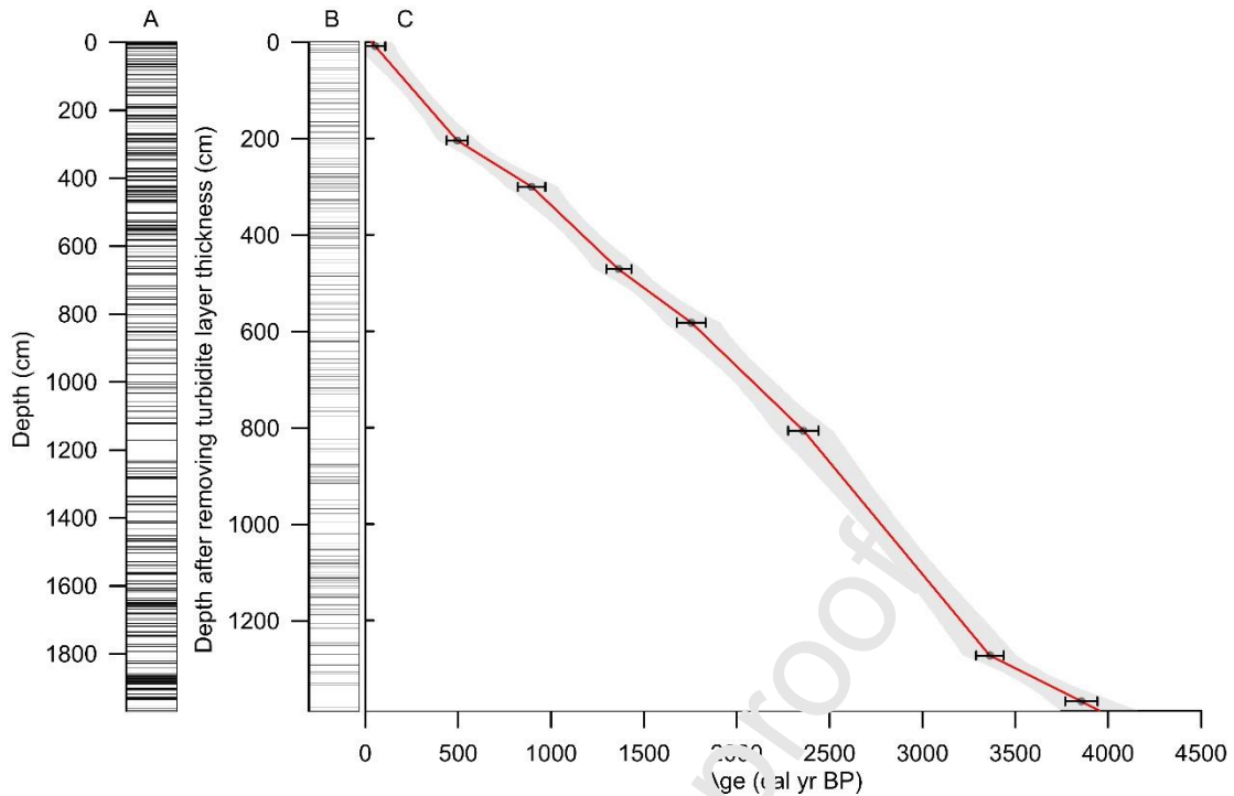
Fig. 4. Age-depth model of Core MD18-3565 in the Gaoqiao Submarine Canyon. (A) Turbidite layer distribution at original core depth scale. (B) Turbidite layer distribution at depth scale after removing turbidite layer thickness. (C) Age-depth model established using the Clam package with linear interpolation. The red line represents the best modelling result and the gray shadow indicates the 95% confidence interval (Blaauw, 2010).
