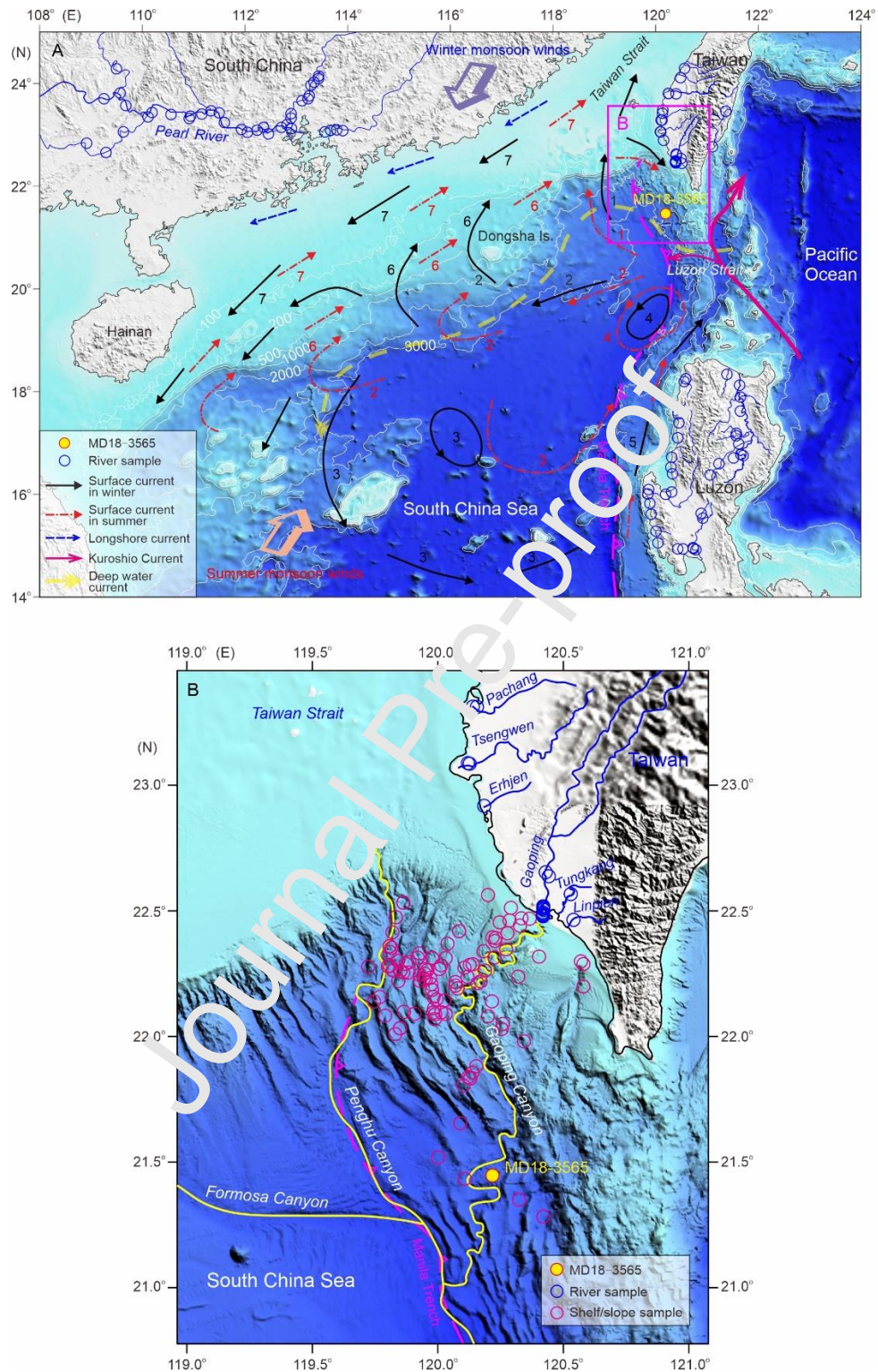
Fig. 1. Topography and oceanography of the northeastern South China Sea (SCS). (A) Current systems and
