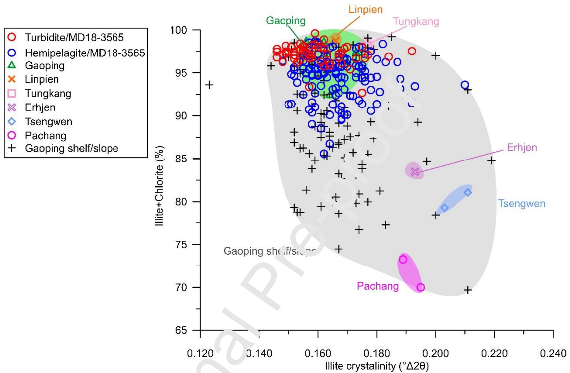
Fig. 11. Contents of illite + chlorite versus illite crystallinity for sediments of Core MD18-3565, and their comparison with Taiwan river and Gaoping shelf/slope sediments (Liu Z et al., 2008, 2010, 2016; Nayak et al., 2021).
