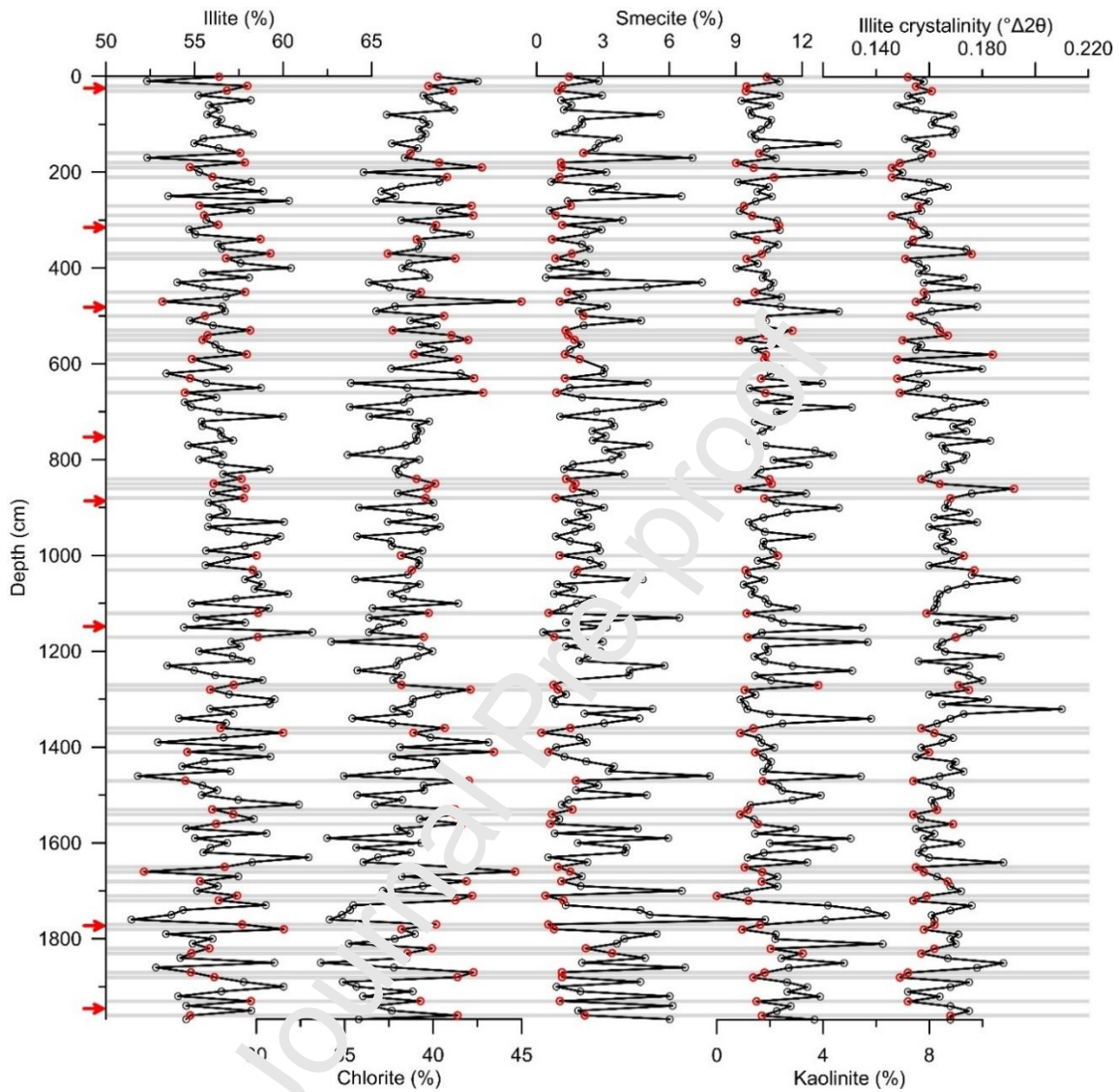
Fig. 5. Depth-scale clay mineral assemblages of Core MD18-3565 in the Gaoping Submarine Canyon. Gray
