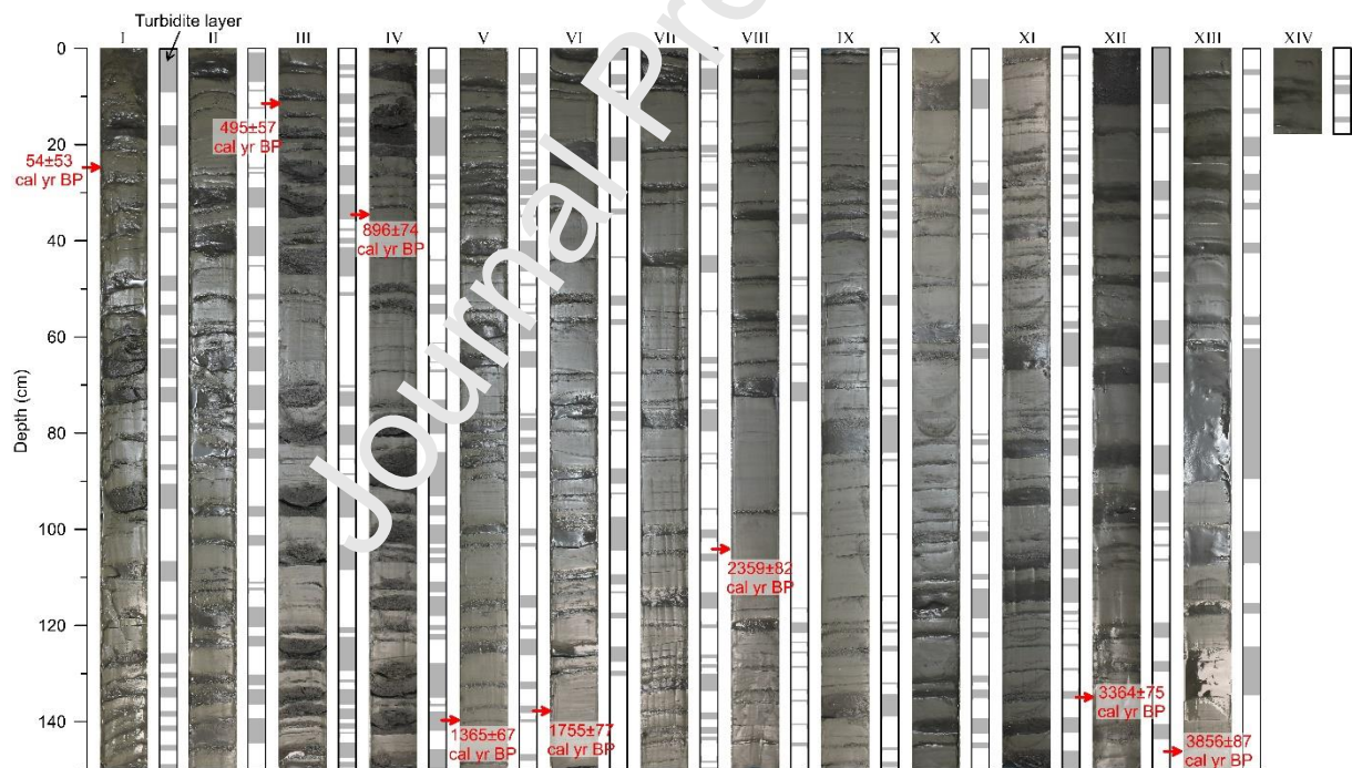
Fig. 2. Core photos and observable turbidite layers (gray bands) of Core MD18-3565 in the Gaoping Submarine Canyon. AMS ^{14}\text{C} dates (Table 2) of planktonic foraminifers and their positions at core sections are indicated. Core photos edited from Colin et al. (2018).
