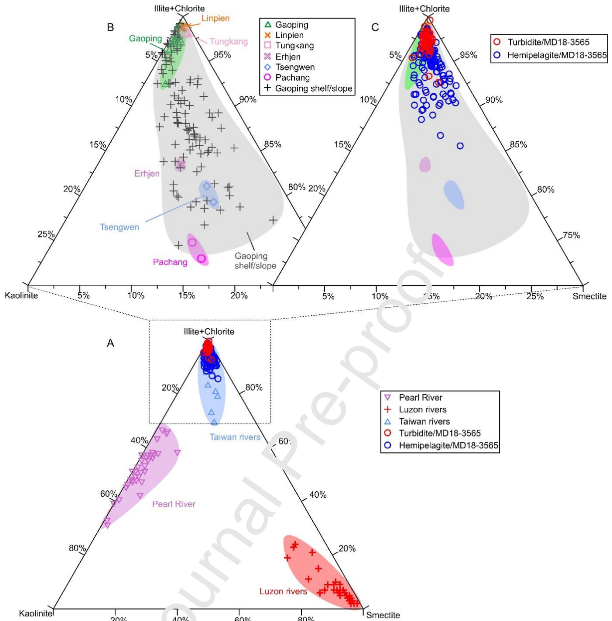
Fig. 10. Ternary diagrams of major mineral groups of illite+chlorite, kaolinite, and smectite. (A) Plots of turbidite and hemipelagite samples of Core MD18-3565. Clay mineral compositions of surface sediments from Taiwan rivers, Luzon rivers, and the Pearl River are included for comparison (Liu Z et al., 2008, 2010, 2016). Square in this panel is zoomed in the panels B and C. (B) Zoomed plots for surface sediments of Taiwan rivers and on Gaoping shelf/slope off southwest Taiwan (Liu Z et al., 2008, 2010, 2016; Nayak et al., 2021). Note that clay mineral compositions of sediment samples from Gaoping, Linpien, and Tungkang rivers are very close to the illite+chlorite end-member, while those of sediments from Erhjen, Tsengwen,
