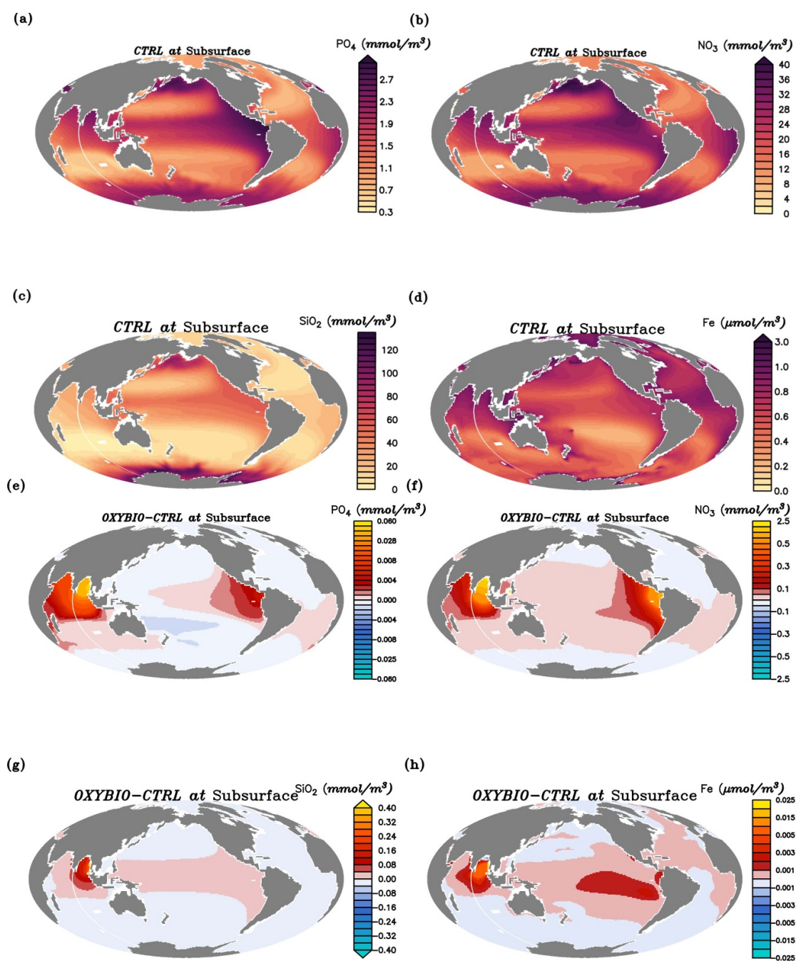
Figure C5. Annual mean subsurface concentrations of phosphate ( \text{PO}_4 ), nitrate ( \text{NO}_3 ), silicate ( \text{SiO}_2 ), iron ( \text{Fe} ) over the last simulated year of the CTRL run (in \text{mmol}/\text{m}^3 and \mu\text{mol}/\text{m}^3 for Fe) (a)–(d). Changes after 100 years of AO injection (OXYBIO-CTRL), of the annual mean subsurface concentrations of these nutrients (e)–(h).
