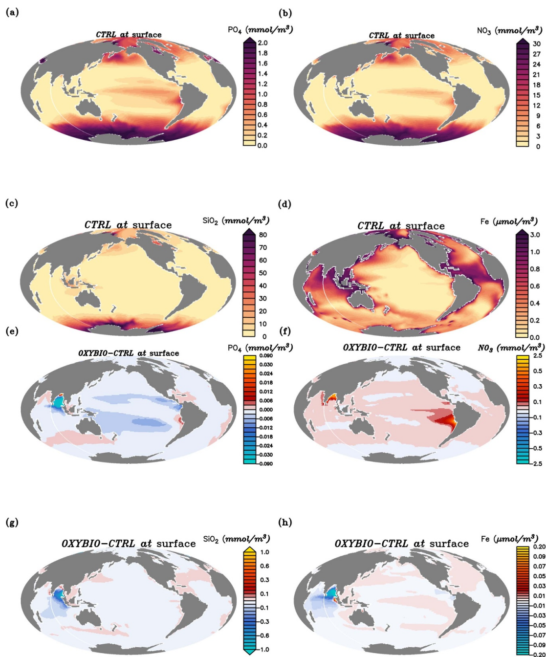
Figure C4. Annual mean surface concentrations of phosphate (PO 4 ), nitrate (NO 3 ), silicate (SiO 2 ), iron (Fe) over the last simulated year of the CTRL run (in mmol m -3 and μmol m -3 for Fe) (a)–(d). Changes after 100 years of AO injection (OXYBIO-CTRL), of the annual mean surface concentrations of these nutrients (e)–(h).
