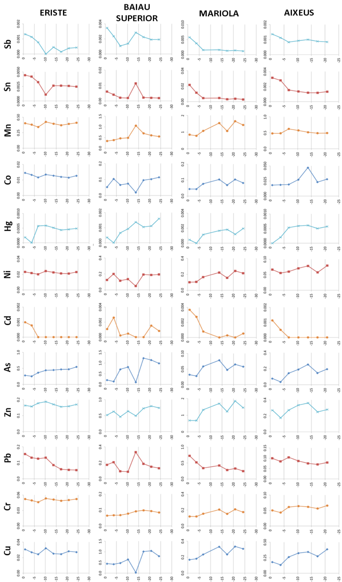
Figure S1 (cont.). Vertical concentration profiles of the elements measured in the sediment cores obtained from Pyrenean lakes. Depth in cm is plotted in axes Y. Concentrations normalised with Ti are plotted in axes X.
