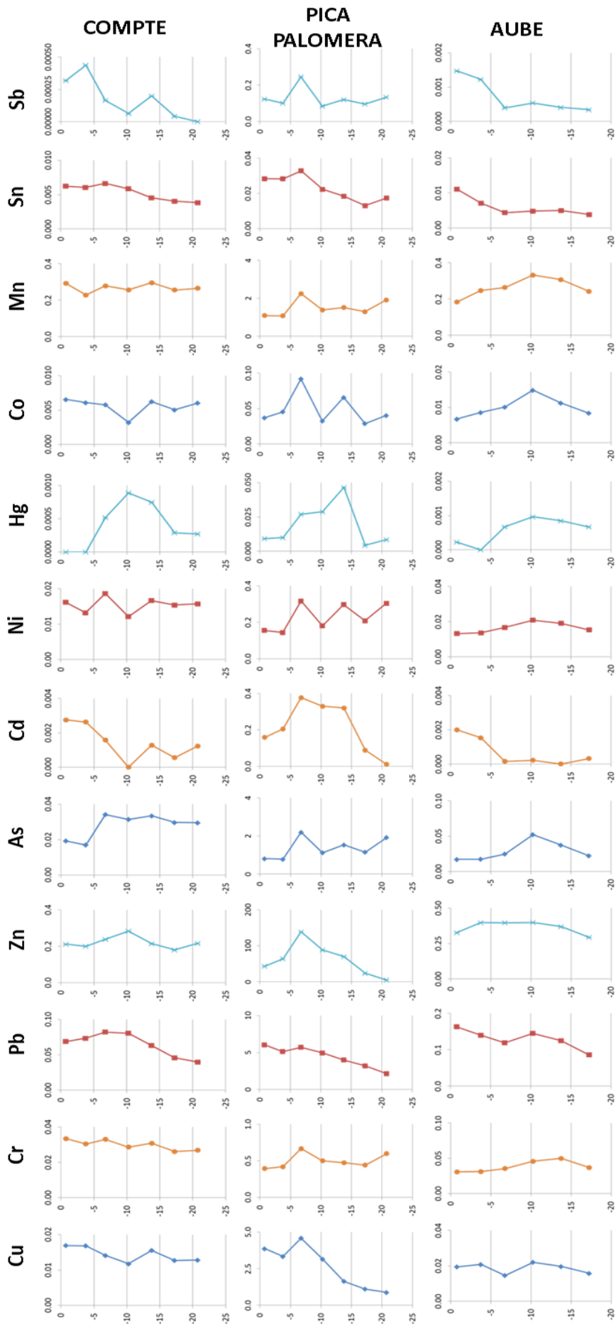
Figure S1 (cont.). Vertical concentration profiles of the elements measured in the sediment cores obtained from Pyrenean lakes. Depth in cm is plotted in axes Y. Concentrations normalised with Ti are plotted in axes X.
