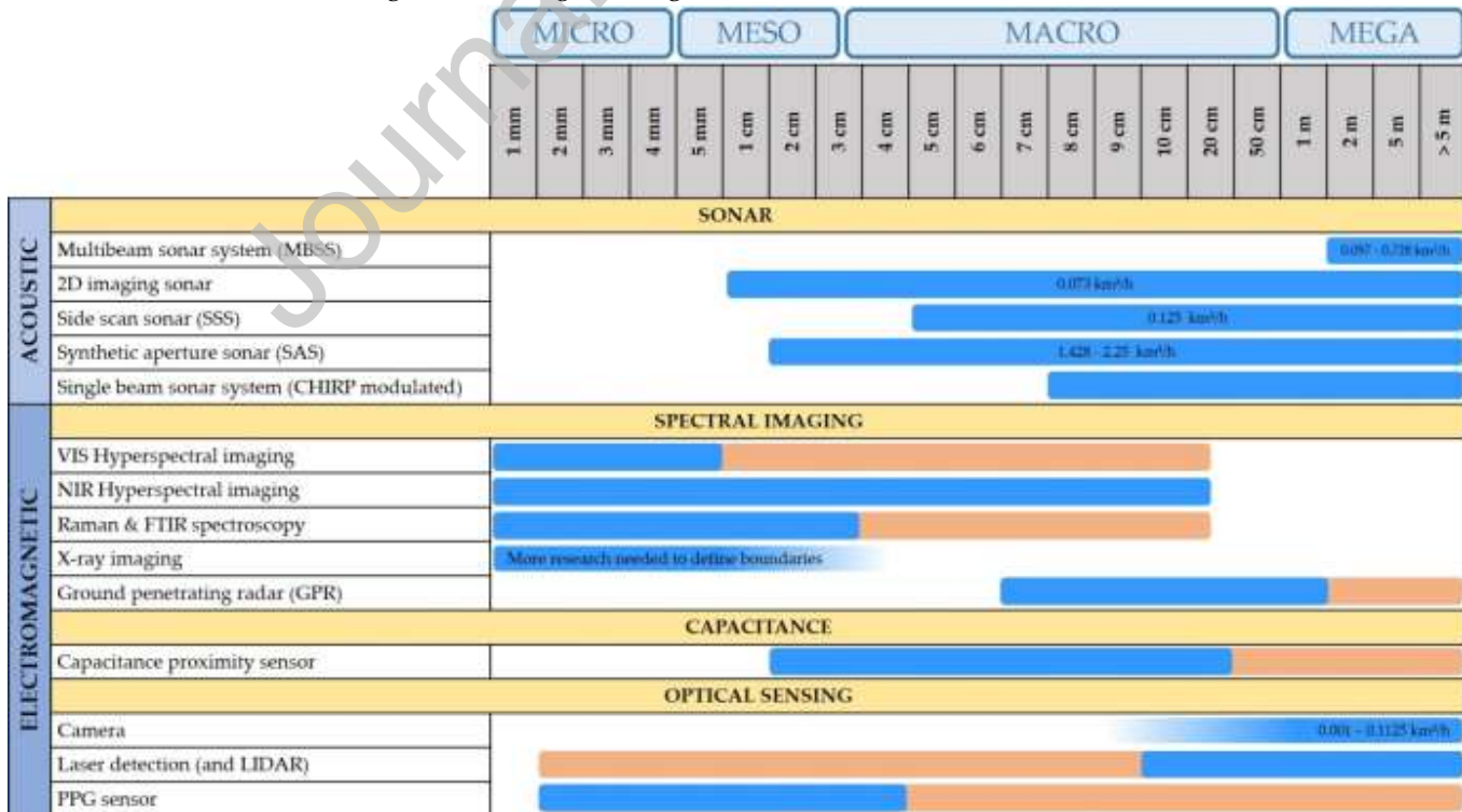
Figure 4. Detection size range and spatial coverage (in km²/h) by seafloor detection technique. Blue bars show the detection range reported in literature to date. Orange bars show the possible extension of size range based on expert judgement of the co-authors.
