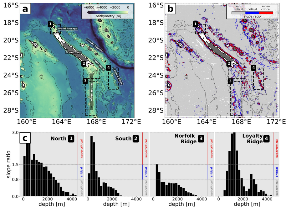
Figure 7. CALEDO60 (a) bathymetry and (b) M2 tide slope ratio \alpha between topographic slope and wave slope s , divided into subcritical (gray, \alpha < 0.8 s ), critical (blue, 0.8 s < \alpha < 1.5 s ), and supercritical (red, \alpha > 1.5 s ) slopes. Note that white shaded grid points are associated with a zero bathymetry gradient. The thin black lines represent the 1000, 2000, and 3000 m depth contours. The thick black line is the 100 m depth contour representative for the New Caledonian lagoon. The numbered black boxes represent the hot spots of internal-tide generation (1: North, 2: South, 3: Norfolk Ridge, 4: Loyalty Ridge) for which the distribution of the slope ratio as a function of depth (divided into 200 m depth bins) is given in (c).
