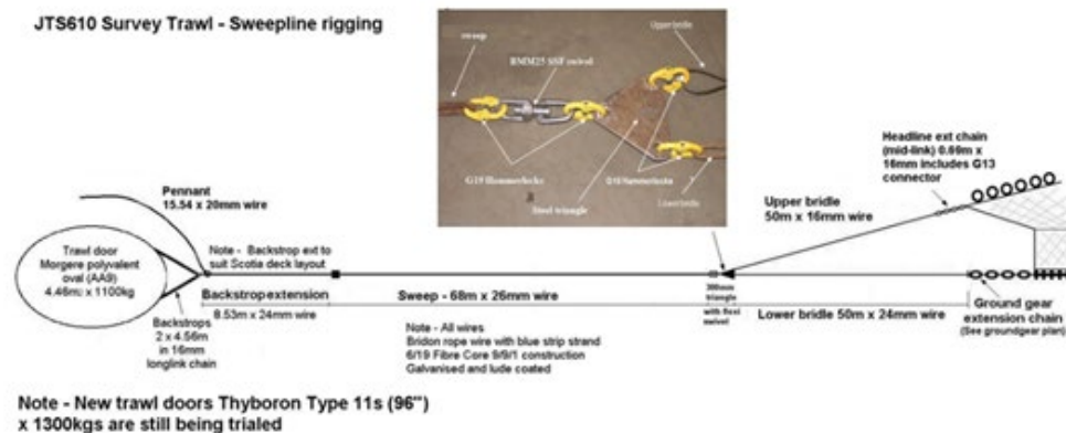
Figure 4.6. Wire rig specification for the proposed trawl.
