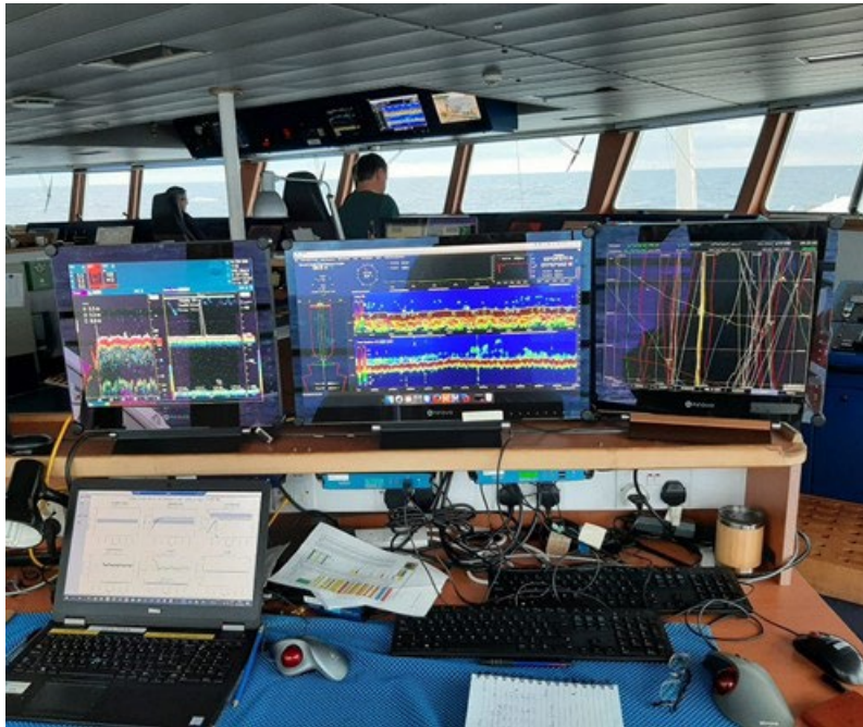
Fig 3.1.3 Aft bench on Celtic Explorer where scientists monitor survey and trawl parameters on a Scanmar bridge unit (top left monitor), MARPORT unit (top middle monitor) and location in proximity to historic commercial and survey data on a Sodena Chart Plotter (top right monitor). A custom application in R to plot and log median values in real-time for the local database thus DATRAS, is running on the laptop.
