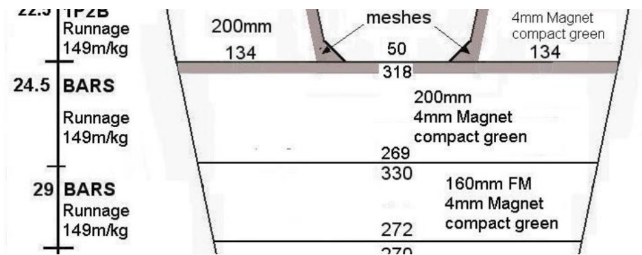
Fig 2.3.1 Top bosom section of the revised BT237.
