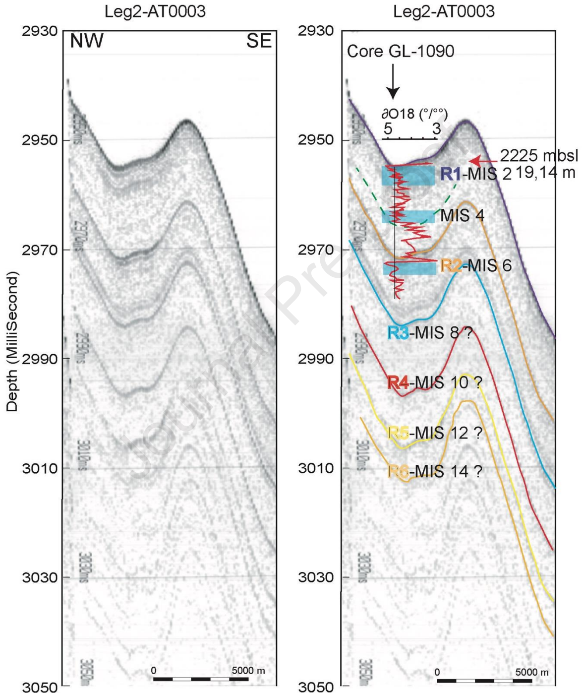
Figure 5: Correlation between SANBA Chirp profile AT003 with core GL 1090 (see location on Figure 1). Depth (cm) in core to (ms) transformation was done using a velocity of 1,600 \text{ m}\cdot\text{s}^{-1} in the sediments.
