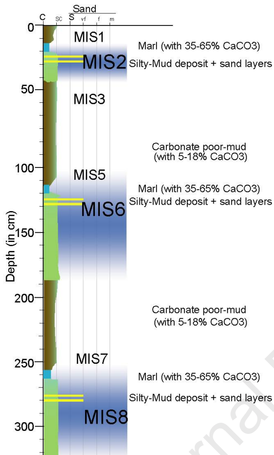
Figure 11 Synthetic characteristics of lithologies from the cores, with Silty-mud and sand layers during Glacial Maxima and marl (35-65% \text{CaCO}_3 ) deposited at transitions between glacial/interglacial followed by carbonate-poor mud.
