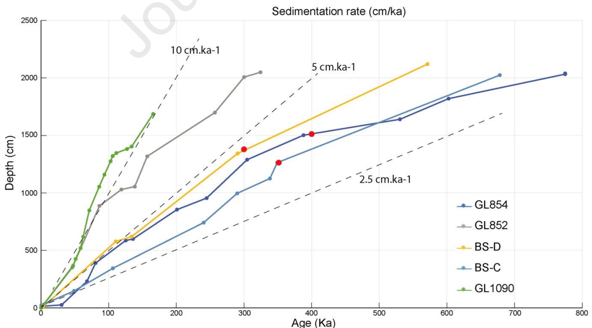
Figure 10: Sedimentation rates from published cores (see Table 1 for references). In dashed black lines constant sedimentation rates (2.5; 5; and 10 cm/ka).
