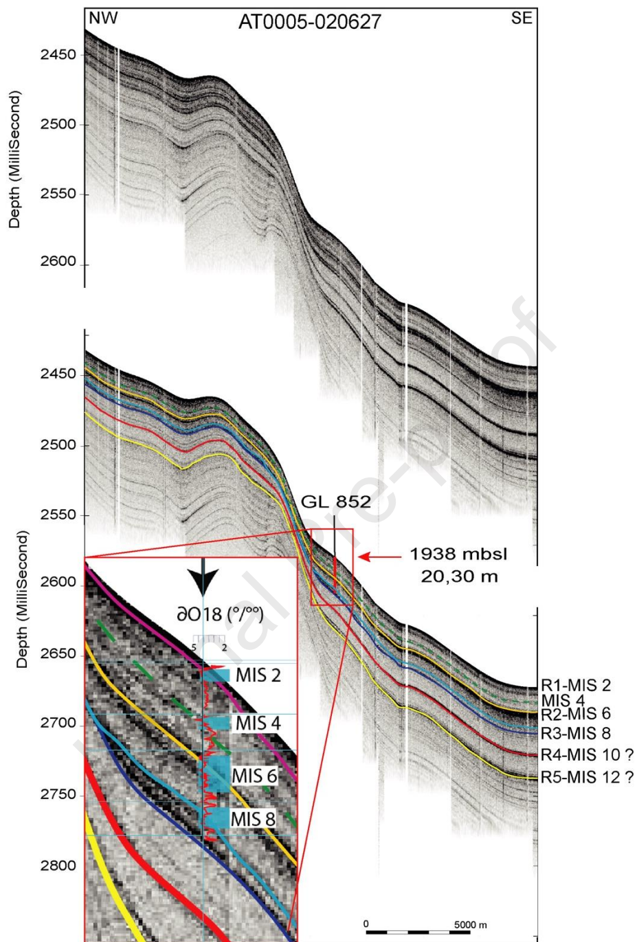
Figure 3: Correlation between SANBA Chirp profile AT0005-020627 and core GL 852 (see location on Figure 1). Depth (cm) in core to (ms) transformation was done using a velocity of 1,600 \text{ m}\cdot\text{s}^{-1} in the sediments.
