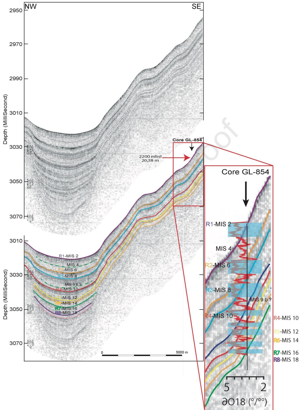
Figure 4: Correlation between SANBA Chirp profile AT003 with core GL 854 (see location on Figure 1). Depth (cm) in core to (ms) transformation was done using a velocity of 1,600 \text{ m}\cdot\text{s}^{-1} in the sediments.
