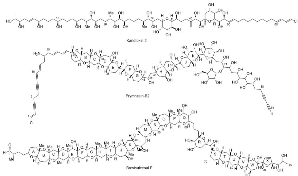
Figure 4.2. Chemical structures of selected microalgal fish killing toxins (Rasmussen et al. 2016).
