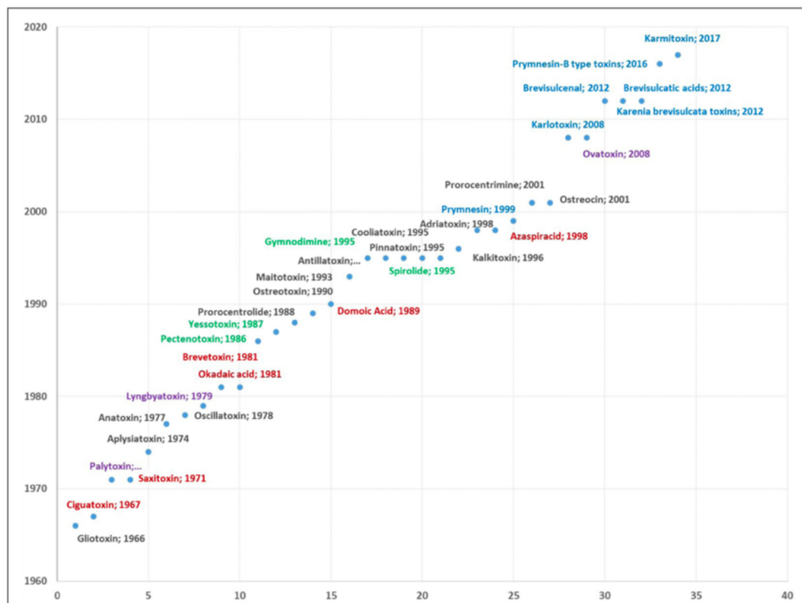
Figure 4.1. Historic overview of discovery and description of the structure of the first analogues of 34 microalgal toxin groups (1966-2017). Color code: blue, toxins involved in fish kills; red, toxins involved in human poisoning; violet, toxins causing skin irritation or respiratory problems (brevetoxins involved in fish kills, human poisoning and skin irritation or respiratory problems); green, toxins known for 20-30 years and not proven to have negative effects on humans or aquatic organisms; black, compounds yet to be related to effects in humans or aquatic biota (adapted from Hess 2018).
