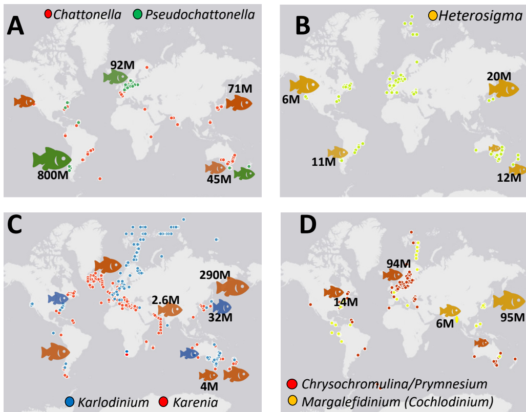
Figure 1.2. Known geographic distributions (from OBIS; as of December 2019) of key fish-killing HAB organisms (coloured dots): A. Chattonella/ Pseudochattonella , B. Heterosigma , C. Karlodinium , Karenia and D. Prymnesium/ Chrysochromulina , Margalefidinium . Fish icons represent exceptionally large economic impacts, indicated by the size of the fish and with economic impacts expressed as million USD damages. Large fish kill events require the incidence of the causative organisms, under favourable environmental conditions, but also the presence of vulnerable aquaculture operations.
