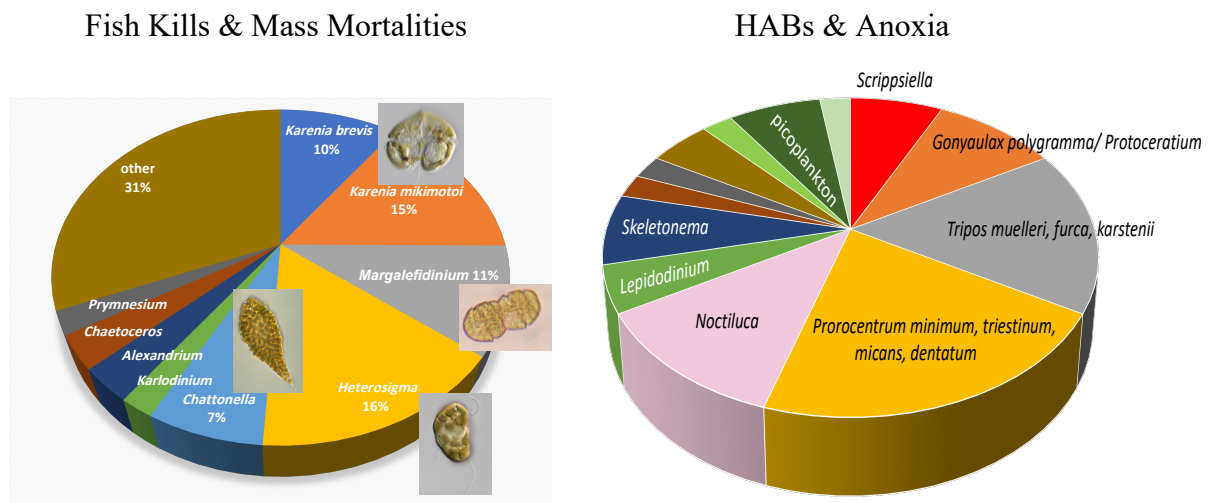
Figure 1.1. Overview of causative organisms of (left) fish kills and mass mortalities and (right) HABs and anoxia (from HAEDAT; as of December 2019).
