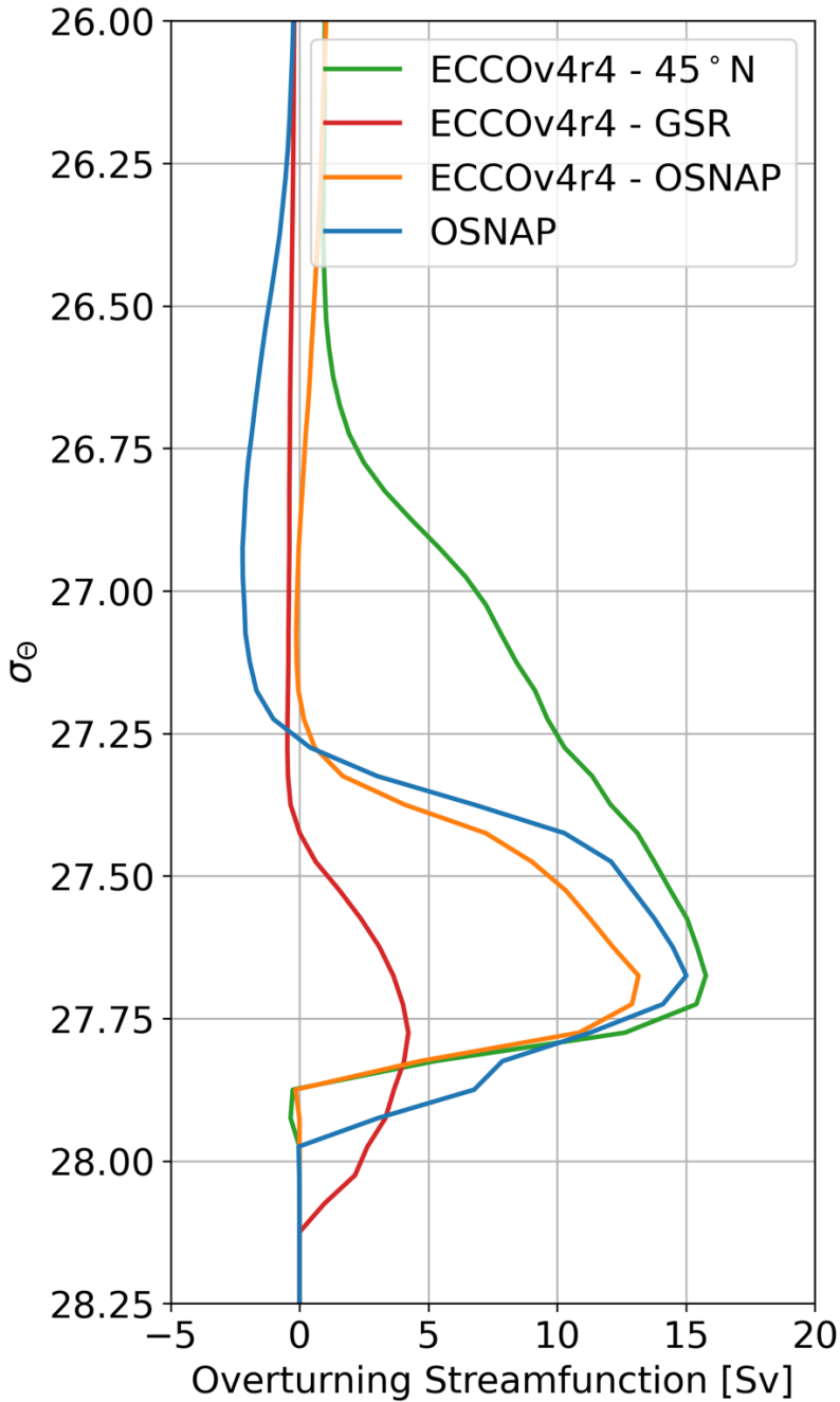
Figure S1: A comparison between the mean Atlantic overturning streamfunction in density space at OSNAP for ECCOv4 (orange) and OSNAP observations (blue). The overturning streamfunction in density space is also shown at 45°N (green) and the Greenland-Scotland Ridge (red). The convergence of the overturning between 45°N (green) and the Greenland-Scotland Ridge is shown in Figure 2a.
