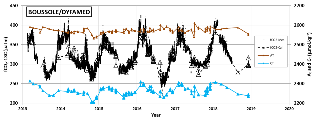
Figure S4: Top: Time-series for the period 2013-2018 of A_T (brown triangles, right Y-axis), C_T (blue triangles, right Y-axis), fCO_2 calculated (open triangles, left Y-axis) and high-frequency fCO_2 measured from CARIOCA (back dotted at 3 and 10m) at the station BOUSSOLE near DYFAMED in the Ligurian Sea (Merlivat et al, 2018; Golbol et al, 2020). For A_T and C_T data are selected in the top layer (0-20m) from BOUSSOLE, DYFAMED and MOOSE-GE samples at the same location. Here fCO_2 is normalized at a temperature 13°C for which the seasonality is mainly driven by C_T (Merlivat et al., 2018; Coppola et al., 2020). Bottom: Measured fCO_2 versus calculated fCO_2 for co-located samples (Dashed line: fCO_2\text{-Carioca} = 1.0341 * fCO_2\text{-Cal} - 9.321 , R^2 = 0.8976 ). The mean difference ( fCO_{2cal} - fCO_{2mes} ) for 67 co-located samples is -3.7 \mu\text{atm} (\pm 10.8) \mu\text{atm} . Localization of the samples is shown in the inserted map (orange circle).
