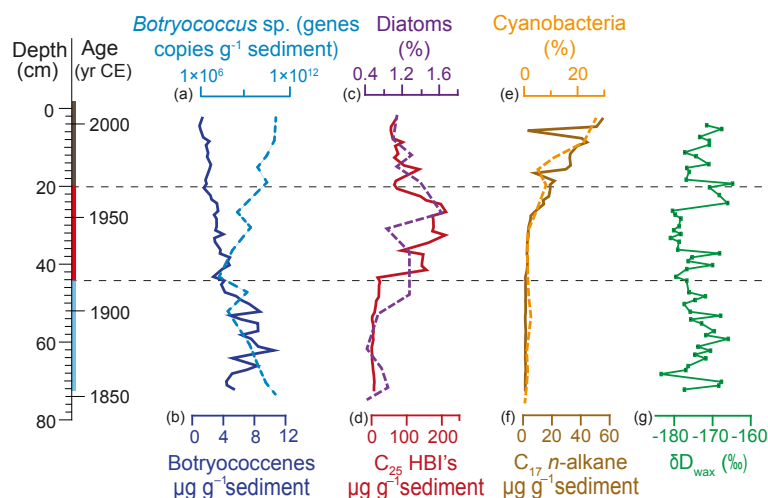
Figure 4. Depth and age profiles of: (a) Botryococcus sp. (18S rRNA genes copies \text{g}^{-1} sediment) (blue dashed), (b) botryococenes, a proxy for Botryococcus braunii (B race) (blue solid), (c) diatoms (%) (purple dashed), (d) \text{C}_{25} Highly branched Isoprenoid (HBIs), a proxy for diatoms (red solid), (e) cyanobacteria (%) (mustard dashed), (f) \text{C}_{17} n -alkane, a proxy for cyanobacteria (brown solid) and (g) \delta D values of \text{C}_{27-29-31} n -alkanes ( \delta D_{\text{wax}} ), a proxy for rainfall amount (green). The black dashed lines represent the transitions between the different units. For interpretation of the references to colour, the reader is referred to the web version of this article.
