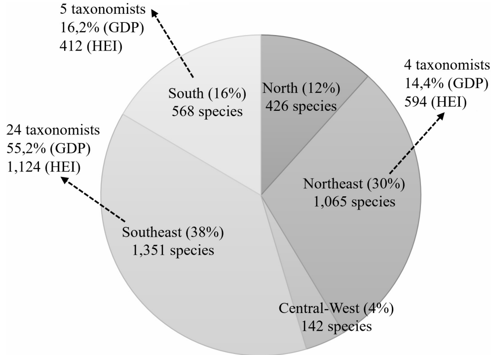
Figure 3. Distribution of 3,552 valid species of Mollusca and malacologists (=taxonomists) by region of Brazil and the possible correlation with socioeconomic indicators. Only the authors of this paper were counted (international authors excluded). (GDP) Gross Domestic Product, (HEI) Higher Education Institutions.
