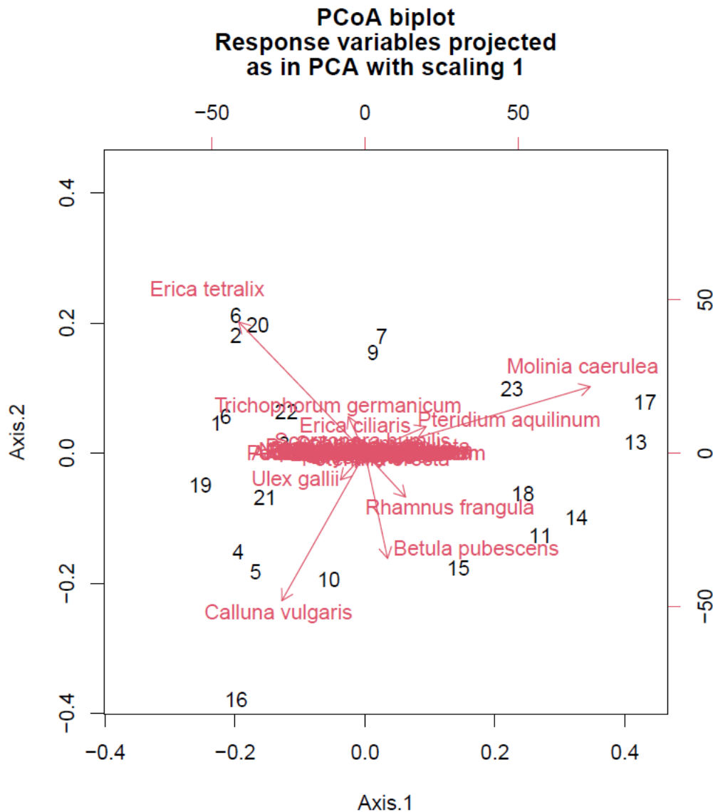
Fig. S1: Principal Coordinate Analysis (PCoA) biplot Response variables projected as in Principal Component Analysis (PCA) with scaling 1.
