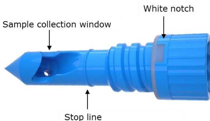
Figure 3. The GST in place on the manual decapper tool, which functions as a handle.
