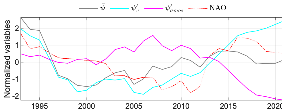
Figure 11: Winter NAO (dotted red line), \bar{\psi} (grey), \psi'_v (cyan) and \psi'_{\sigma_{moc}} (magenta). Time series were normalized by their standard deviations and low-pass filtered using a moving mean with a 60-month window.
