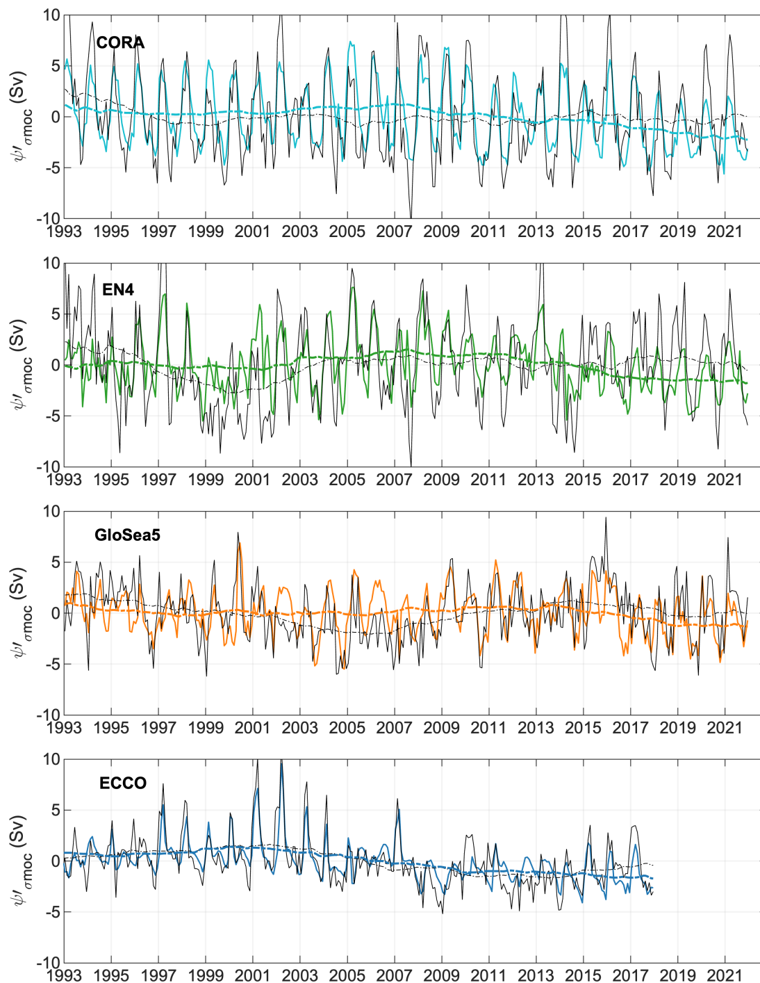
Figure 6 : Coloured solid lines are times series of \psi'_{\sigma_{moc}} in Sv for CORA (cyan), EN4 (green), GloSea5 (orange) and ECCO (blue). The black solid lines are \psi' . The coloured (black) dashed lines are \psi'_{\sigma_{moc}} ( \psi' ) after low-pass filtering with a moving average of 60 months.
