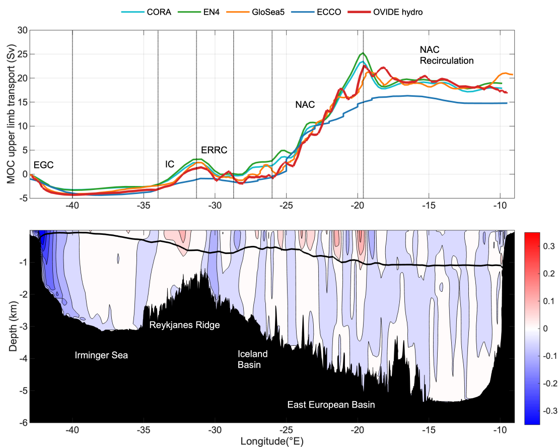
295 Figure 3: (upper panel) Cumulated transport from Greenland to Portugal along the OVIDE line in the MOC upper limb in Sv for CORA (cyan), EN4 (green), GloSea5 (orange) and ECCO (blue) averaged over the time period covered by the cruises, and the average of the 1997–2018 OVIDE hydrographic line (red). (lower panel) geostrophic velocity ( \text{m s}^{-1} ) perpendicular to the OVIDE line averaged over the OVIDE cruises and adapted from Danault et al. (2016). Positive velocities are directed northwards. The continuous black line is \sigma_{\text{moc}} averaged over the OVIDE cruises. Main bathymetric features are indicated. EGC stands for East Greenland Current, IC for Irminger Current, ERRC for East Reykjanes Ridge Current, NAC for North Atlantic Current, with the dotted vertical lines indicating the extension in longitude of the currents. 300
