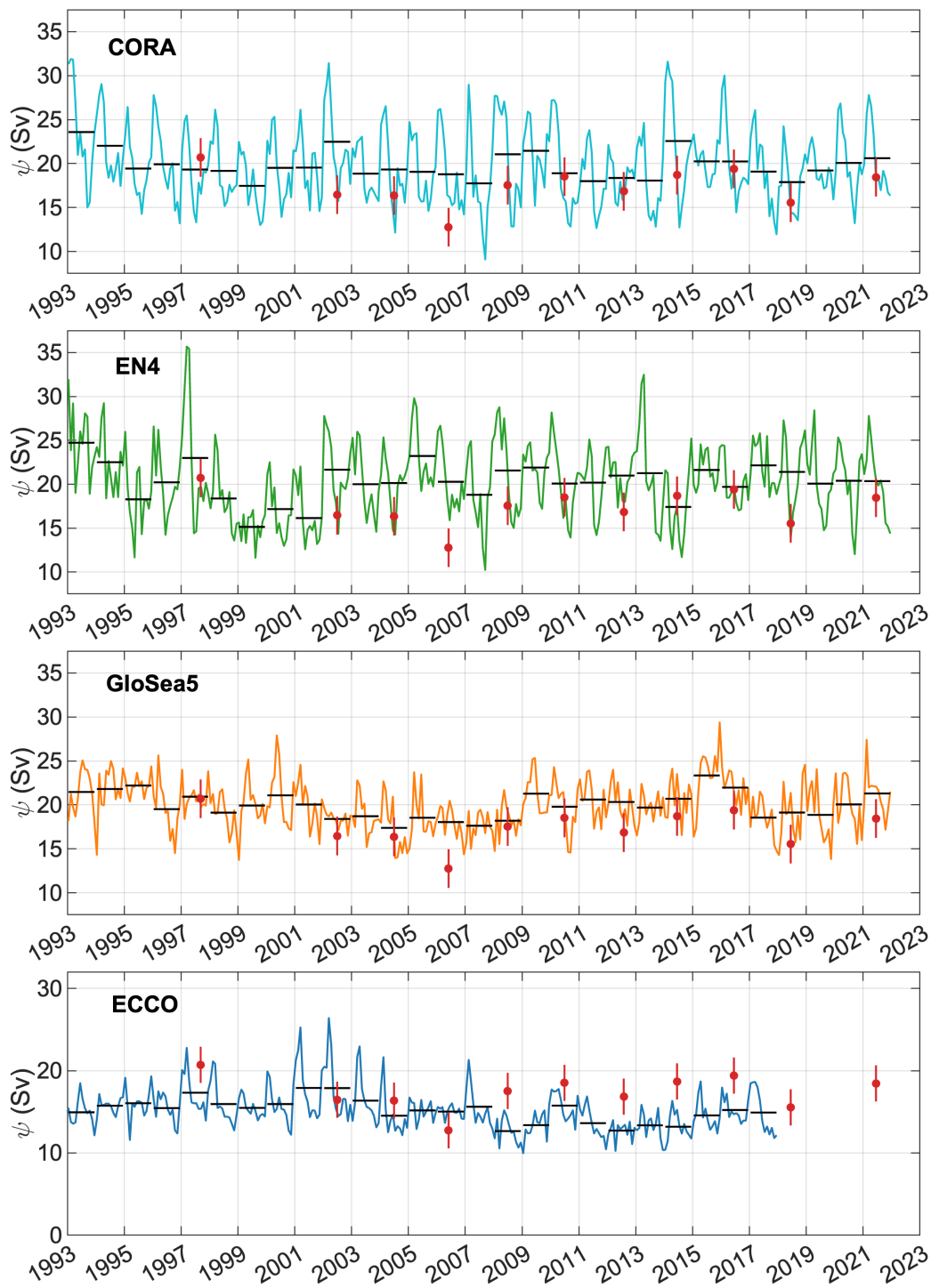
Figure 2: Time series of MOC strength at OVIDE from CORA (cyan), EN4 (green) and GloSea5 (orange) and ECCO (blue) in Sv. MOC strengths and associated standard errors estimated from OVIDE hydrographic lines are plotted in red. The annual means of each time series (black, horizontal lines) are also indicated.
