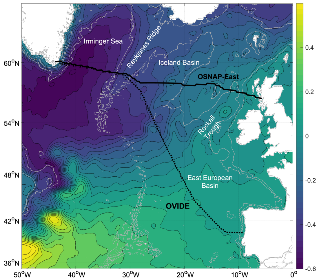
75 Figure 1: OVIDE and OSNAP East lines plotted over the mean sea surface height (m) from AVISO. The 200 and 2000 meters isobaths are plotted in grey.
