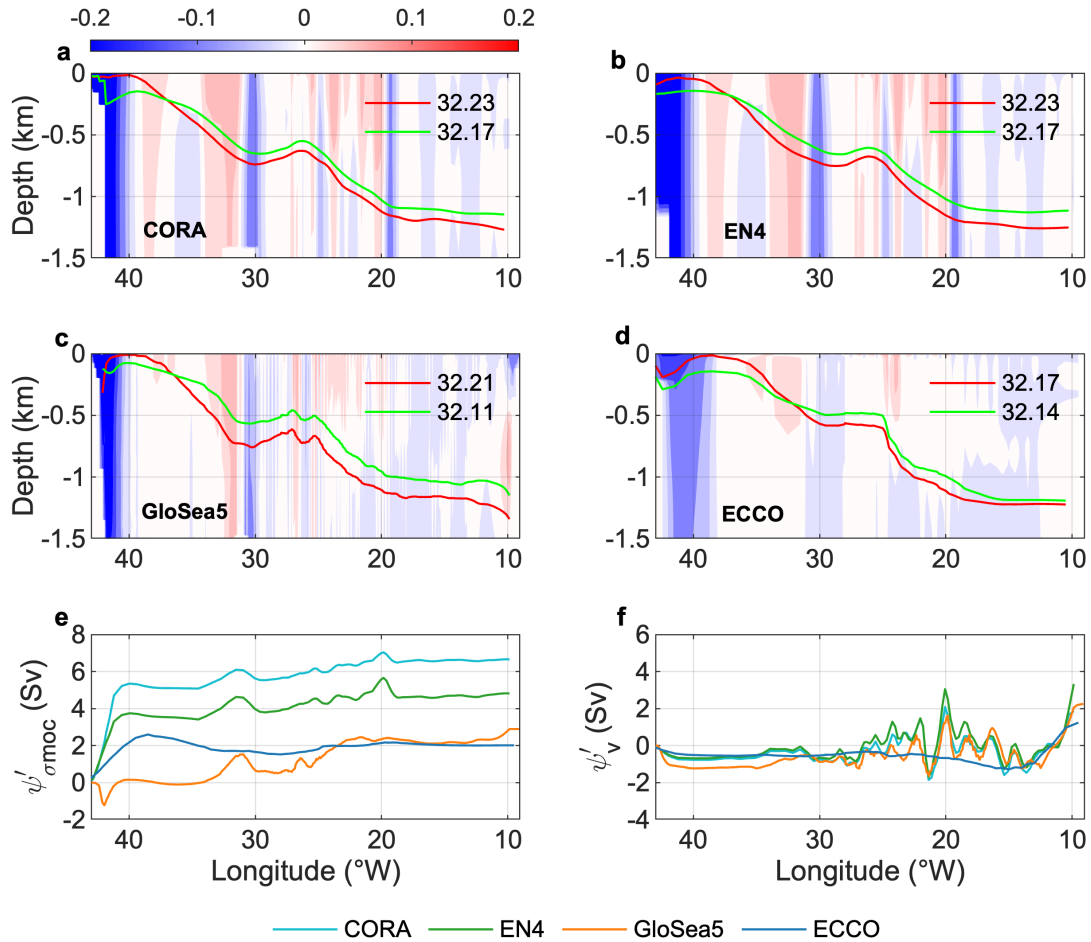
405 Figure 8 : The longitude evolution of \sigma_{moc} depths averaged over February–April (red, maximum of \psi seasonal cycle) and September– November (green, minimum of \psi seasonal cycle) for (a) CORA, (b) EN4, (c) GloSea5 and (d) ECCO from Greenland to Portugal. The background field is the velocity perpendicular to the OVIDE line in m s^{-1} . Legend in panels a-d is density of \sigma_{moc} . (e) Transport anomalies corresponding to the difference between the 3-month average at the maximum and minimum of \psi'_{\sigma_{moc}} seasonal cycle (February–April minus September–November) for \psi'_{\sigma_{moc}} . (f) Transport anomalies corresponding to the difference between the 3- month average at the maximum and minimum of \psi'_v seasonal cycle (October–November minus July–August). Transport anomalies 410 are reported in Sv and accumulated eastward from the Greenland coast in the upper limb of the MOC for \psi'_{\sigma_{moc}} (e) and \psi'_v (f).
