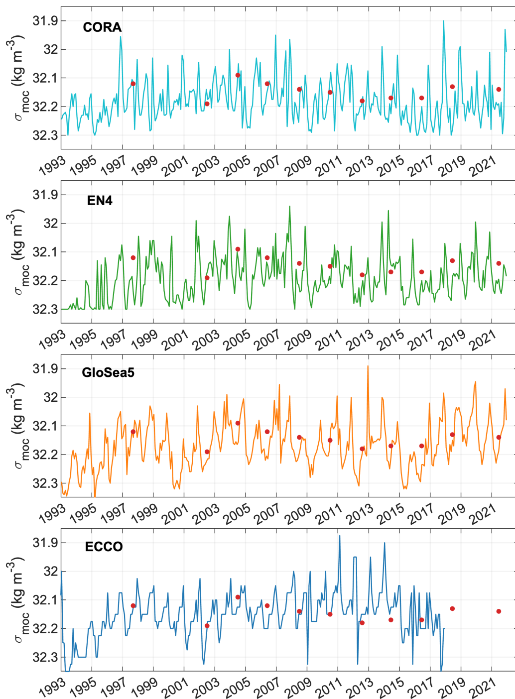
Figure 4 : Times series of potential density reference to 1000 dbar at the maximum of the overturning stream function ( \sigma_{moc} ) in \text{kg m}^{-3} for CORA (cyan), EN4 (green) and GloSea5 (orange) and ECCO (blue). \sigma_{moc} from OVIDE hydrographic lines are plotted as red dots.
