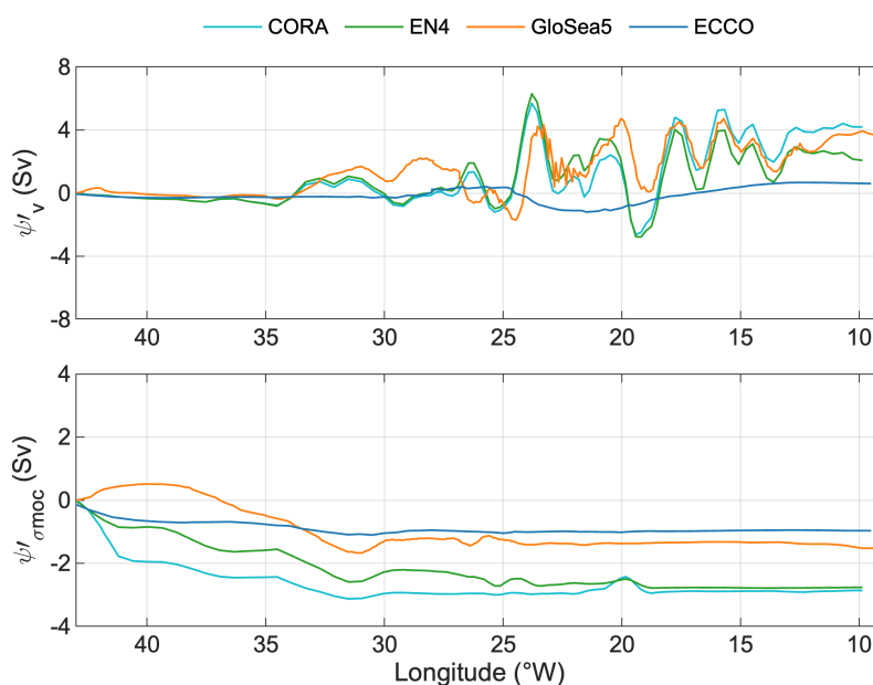
455 Figure 10: Transport difference (Sv) between 2015–2018 and 2004–2008 accumulated in the MOC upper limb from the western boundary eastward along the OVIDE line for \psi'_v (upper panel) and \psi'_{\sigma_{moc}} (lower panel). CORA is reported in cyan, EN4 in green, GloSea5 in orange and ECCO in blue.
