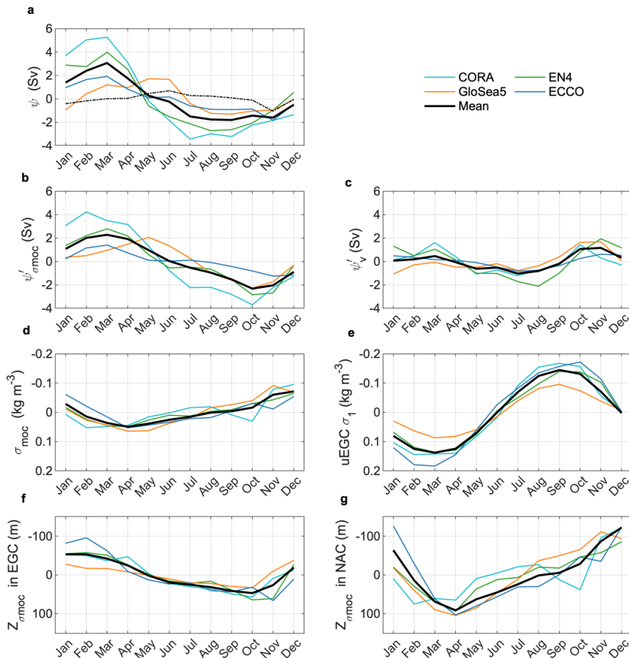
400 Figure 7 : Mean intra-annual variability of (a) MOC \psi' at OVIDE in Sv, (b) \psi'_{\sigma_{moc}} , (c) \psi'_v , (d) \sigma_{moc} in \text{kg m}^{-3} , (e) \sigma_1 in the upper EGC (100-300 m), (f) Z_{\sigma_{moc}} in the EGC defined as the southward flowing western boundary current west of 40°W (Figure 3), (g) Z_{\sigma_{moc}} in the NAC defined as the broad current system east of 26°W (Figure 3). Each panel shows CORA (cyan), EN4 (green), GloSea5 (orange), ECCO (blue) and the mean of all 4 analyses. Black-dashed line in (a) is the Ekman transport, common to all analyses.
