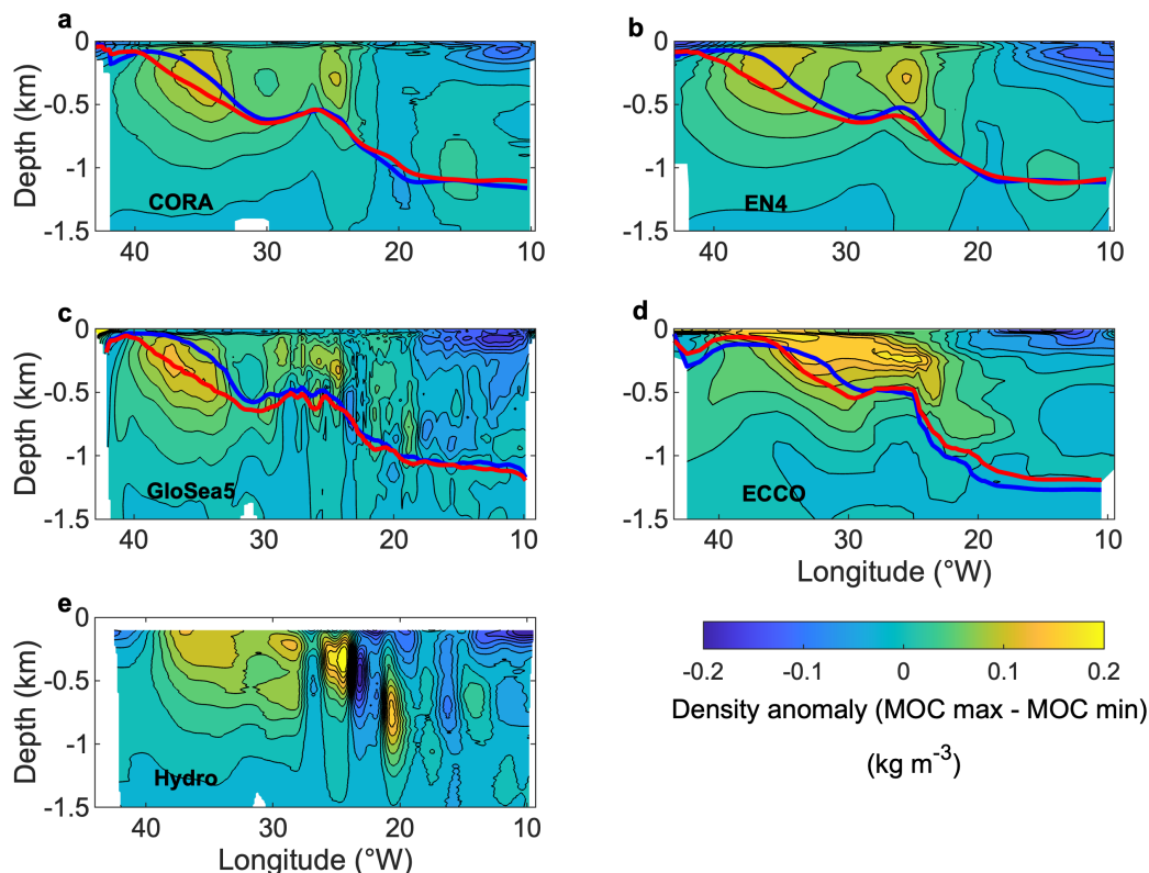
425 Figure 9: Density difference ( \text{kg m}^{-3} ) between 2015–2018 and 2004–2008 for CORA (a), EN4 (b), GloSea5 (c), ECCO (d) and OVIDE hydrography (e) for 0–1500 m along the OVIDE line (Figure 1). The longitude evolution of \sigma_{moc} depths averaged over 2015–2018 (blue solid line) and 2004–2008 (red solid line) are superimposed for panels a–d. For the OVIDE hydrography, the density difference was calculated from the cruise data and smoothed horizontally using a moving average of 70 km to remove noise due to the snapshot nature of the data. Only the density difference for depths less than -0.1 km are plotted to avoid the seasonal aliasing affecting both the surface layer and the \sigma_{moc} depth.
