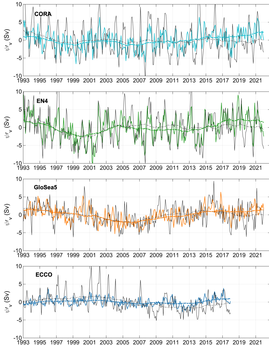
345 Figure 5 : Coloured solid lines are times series of \psi'_v in Sv for CORA (cyan), EN4 (green), GloSea5 (orange) and ECCO (blue). The black solid lines are \psi' . The coloured (black) dashed lines are \psi'_v ( \psi' ) after low-pass filtering with a moving average of 60 months.
