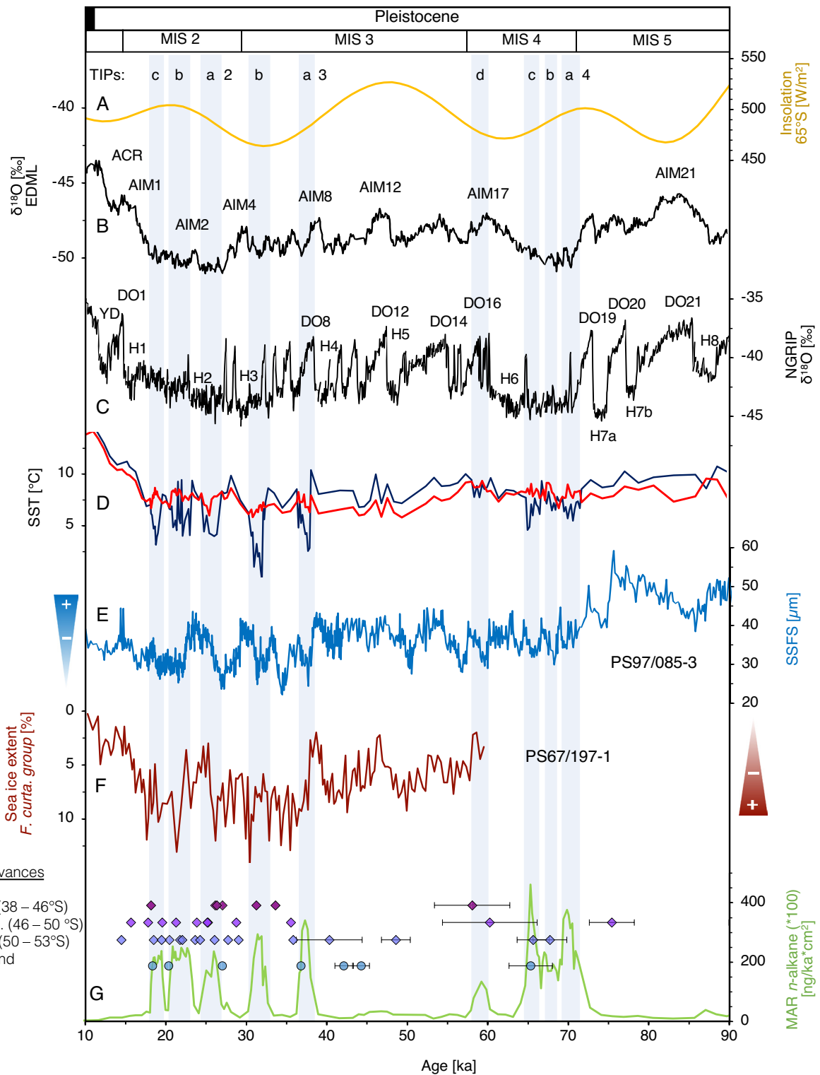
Fig. 4. Detailed view of glacial advances between 90 and 10 ka. Gray stripes and numbers at the top mark terrigenous input phases (TIP). (A) SH summer insolation at 65°S in W/m 2 (72). (B) δ 18 O record from the EDML ice-core (40). ACR = Antarctic Cold Reversal, LIG = Last Interglacial, AIM = Antarctic Isotope Maxima. (C) δ 18 O ice core NGRIP with Dansgaard-Oeschger (DO), Heinrich Events (H) and Younger Dryas [YD; (73)]. (D) Alkenone-derived SSTs, based on U K 37 -index (blue) and U K 37 -index (red). (E) ACC strength reconstruction from the Drake Passage is based on the sortable silt/fine sand (SSFS) of core PS97/085-3 (71). (F) Winter sea ice extent in the Scotia Sea (PS67/197-1) based on the diatom group Fragilariopsis curta (71). (G) The mass accumulation rate of n -alkanes with individual glacier advances of Patagonia (Pat.) and New Zealand. Advances from North Patagonia were taken from refs. 15 and 22. Advances from Central Patagonia were taken from refs. 11–13. Advances from South Patagonia were taken from refs. 6, 7, 10, and 42. Advances from New Zealand were taken from refs. 43 and 44. Literature ages are found in SI Appendix, Table S4 .
