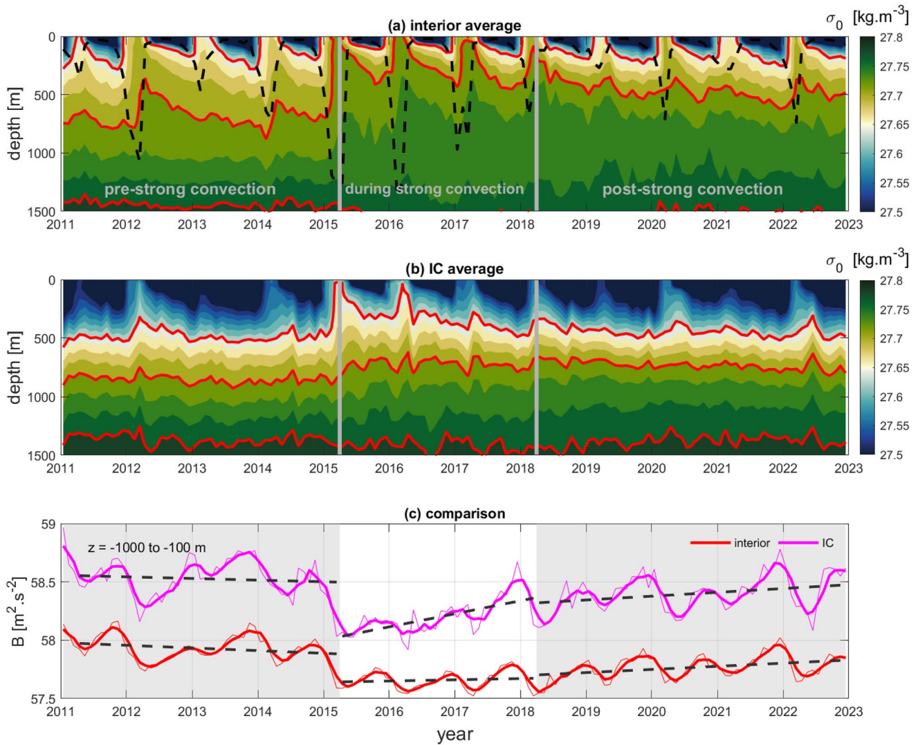
Figure 2. Time-series of the area-averaged potential density in the (a) interior and (b) Irmingier Current (IC) (see Figure 1a for locations), in the upper 1,500 m with the 27.64, 27.72, and 27.78 \text{kg}\cdot\text{m}^{-3} isopycnals overlain (red). The mixed layer depth (black dashed) is shown in (a). (c) Depth-integrated buoyancy content over the 100–1,000 m layer for the interior (red) and IC (pink); thin lines show the raw monthly time-series, thick lines show the smoothed time-series after applying a 4-month moving mean. Thick black dashed lines show linear trend from Least Squares fit for each period.
