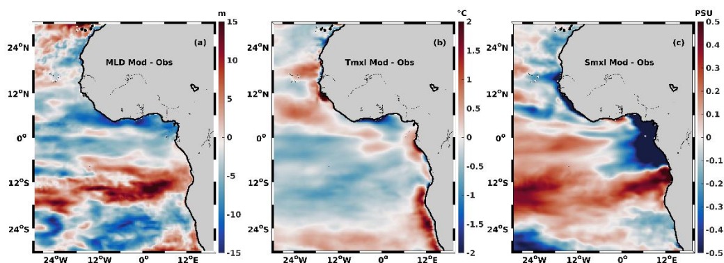
615 Figure A.1: Difference between observations and model in mixed-layer depth (a), mixed-layer temperature (b) and mixed-layer salinity (c).
