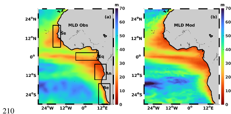
Figure 1: Annual mean of mixed-layer depth from observations (a) and model (b). The rectangles in (a) correspond to the 4 regions of study.
