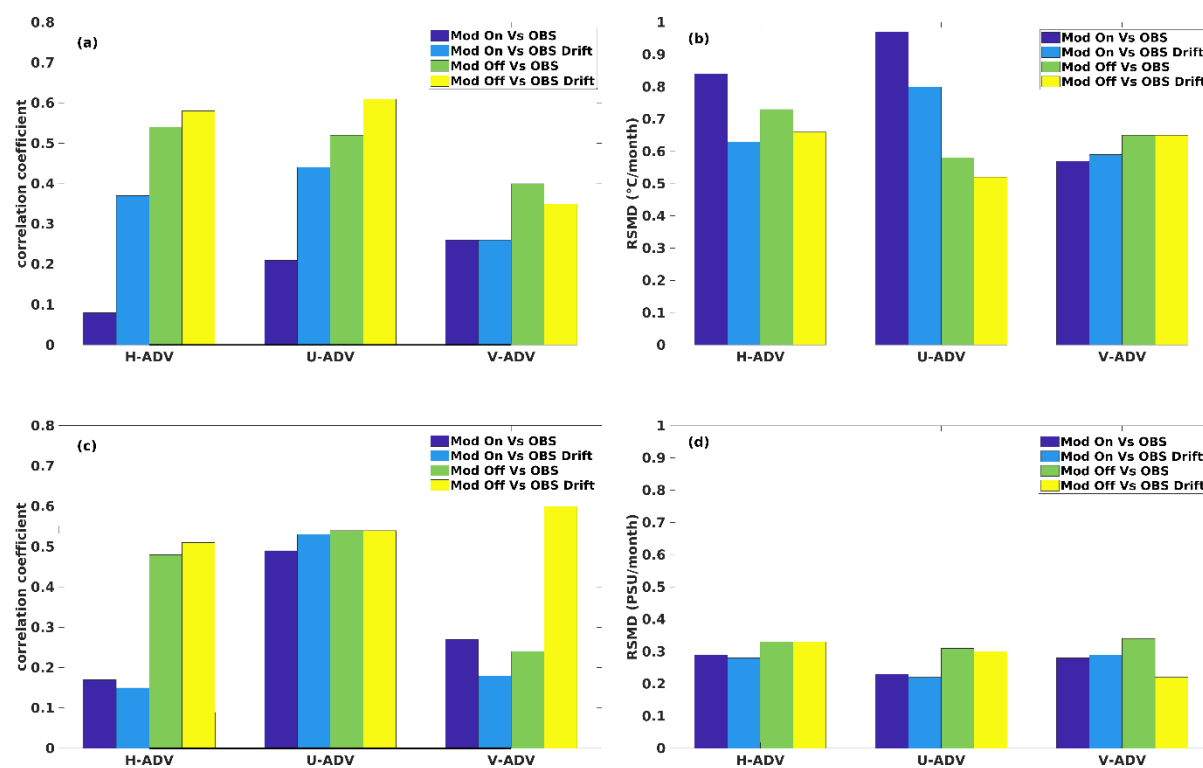
Figure A.2: Spatial correlation ( r ), RMSD of horizontal, zonal and meridional heat (a and b)/salt (c and d) advection between observations (Obs and Obs Drift) and model (online and offline).
