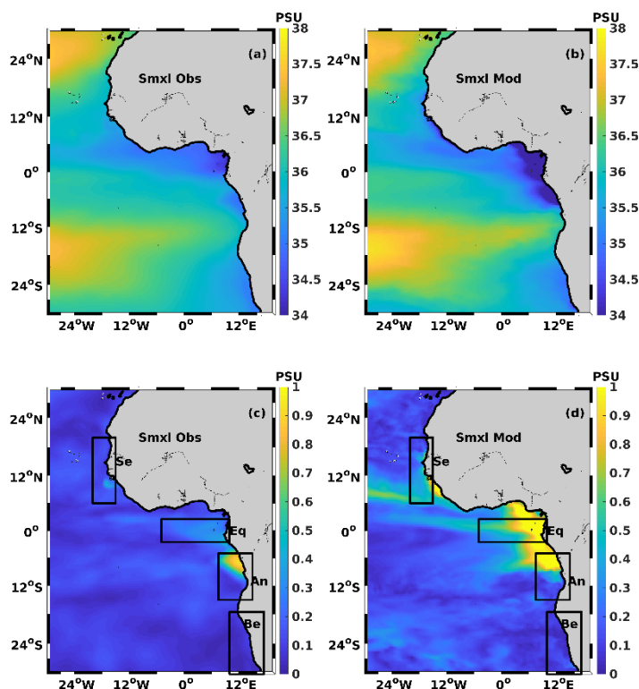
Figure 3: Annual mean (a and b) and standard deviation (c and d) of mixed-layer salinity from observations (left: a and c) and model (right: b and d). The rectangles in the bottom panels correspond to the 4 boxes of study.
