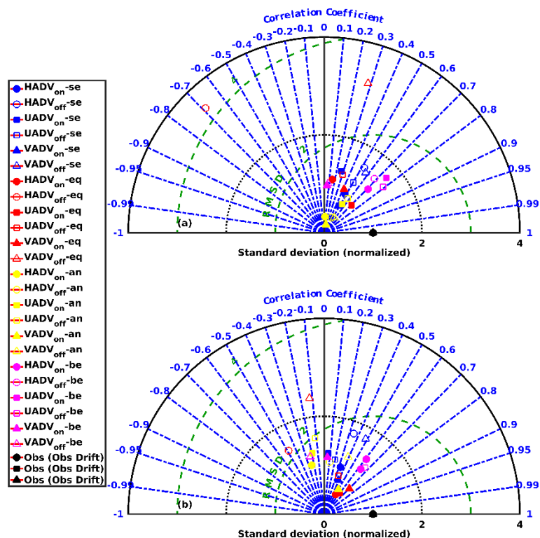
620 Figure A.3: Taylor diagrams comparing seasonal variations of horizontal/zonal/meridional heat advection (HADV/UADV/VADV) from observations (gridded advection named Obs (a) ; Lagrangian advection named Obs Drift (b)) and model (online advection for ON and offline advection for OFF) in Senegal, Equatorial, Angola and Benguela boxes (blue, red, yellow and magenta colors respectively).
