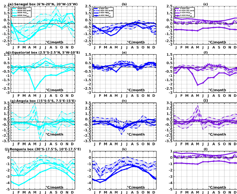
625 Figure A.4: Seasonal cycle of horizontal (cyan), zonal (blue), and meridional (purple) heat advection from observations (dashed line for gridded advection and dotted line for Lagrangian advection) and model (full line for online and full dotted line for offline) in selected boxes. All others terms are in °C per month.
