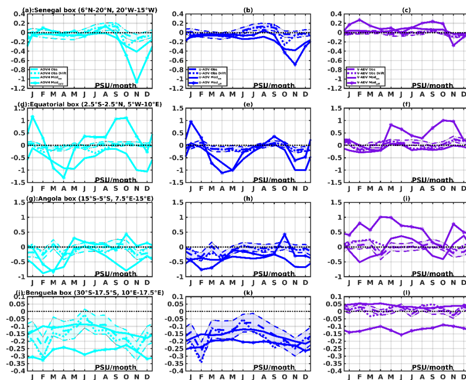
Figure A.6: Seasonal cycle of horizontal (cyan), zonal (blue), and meridional (purple) salt advection from observations (dashed line for gridded advection and dotted line for Lagrangian advection) and model (full line for online and full dotted line for offline) in selected boxes. All other terms are in \text{Psu/month} .
