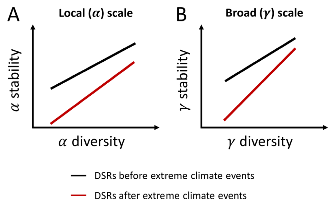
FIGURE 2 Hypothetical changes in diversity–stability relationships (DSRs) at multiple spatial scales before and after an extreme climate event. (A) After an extreme climate event, the strength of DSRs may be increased at the local ( \alpha ) scale due to an increased facilitation among species. (B) These changes in DSRs can propagate to the broader ( \gamma ) spatial scale. With an amplified relationship between spatial asynchrony and \beta diversity, which are additional partitioning products scaling DSRs from local to broader spatial scales, the strength of the DSRs might experience further buffering at the broader ( \gamma ) spatial scale. Black and red lines indicate DSRs before and after extreme climate events, respectively. Information about alternative hypotheses is provided in Appendix S1: Figure S1.
