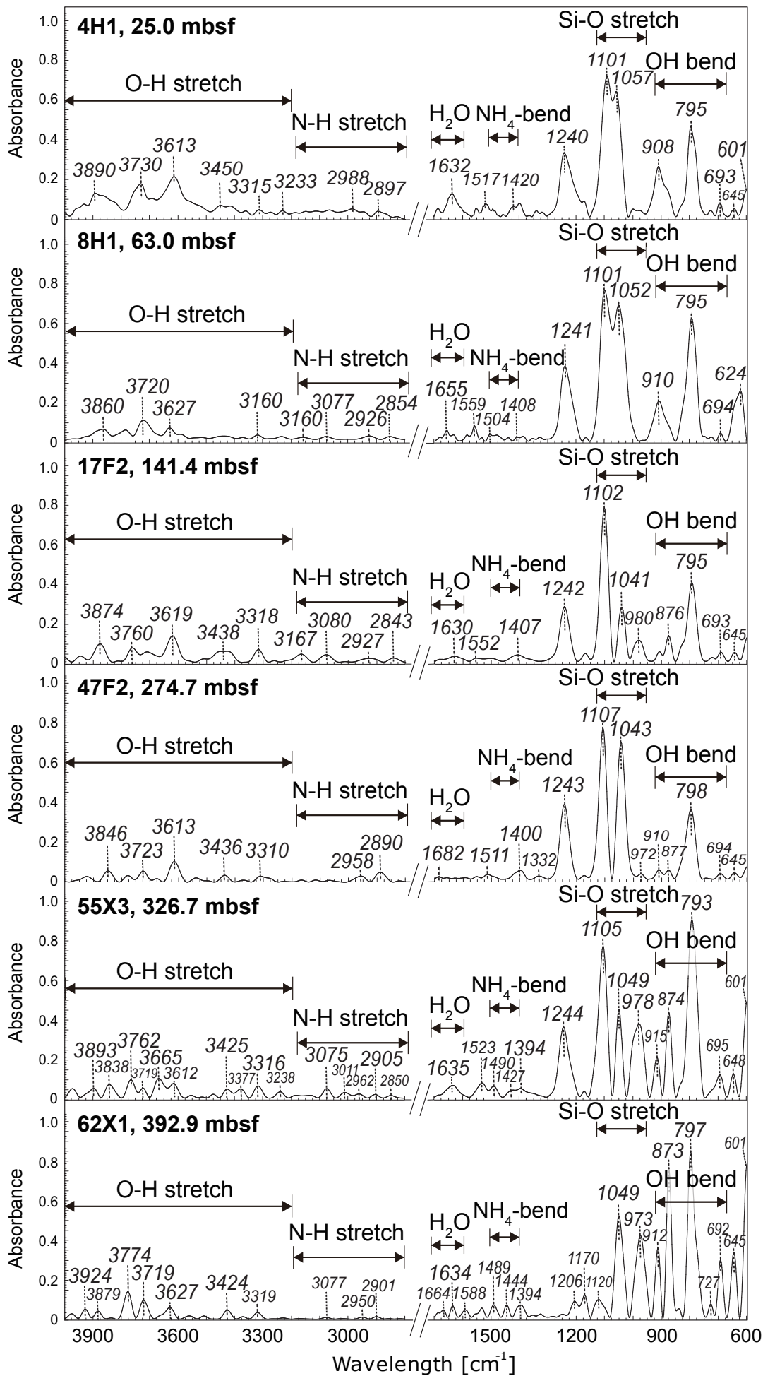
Fig. S3 FT-IR spectra of the bulk sediment samples from the Hole U1545A.
