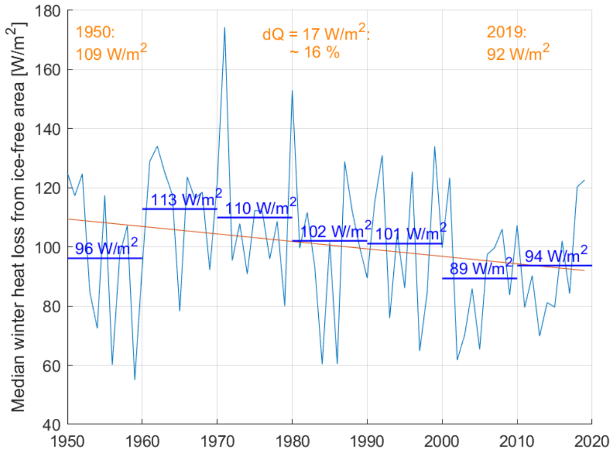
Figure S1.1: Development of per-area heat loss between 1950 and 2019. The blue line represents the median winter heat loss from the ice-free area (sea-ice concentration < 15%) for each winter. The short, dark-blue lines are the mean values for the indicated 10-year periods, mean values are stated above each line. The linear-regression line is shown in orange. Regression values from the beginning and end of the 70-year period were extracted (orange text in upper corners) and their difference is given at the top center of the figure (dQ, orange).
